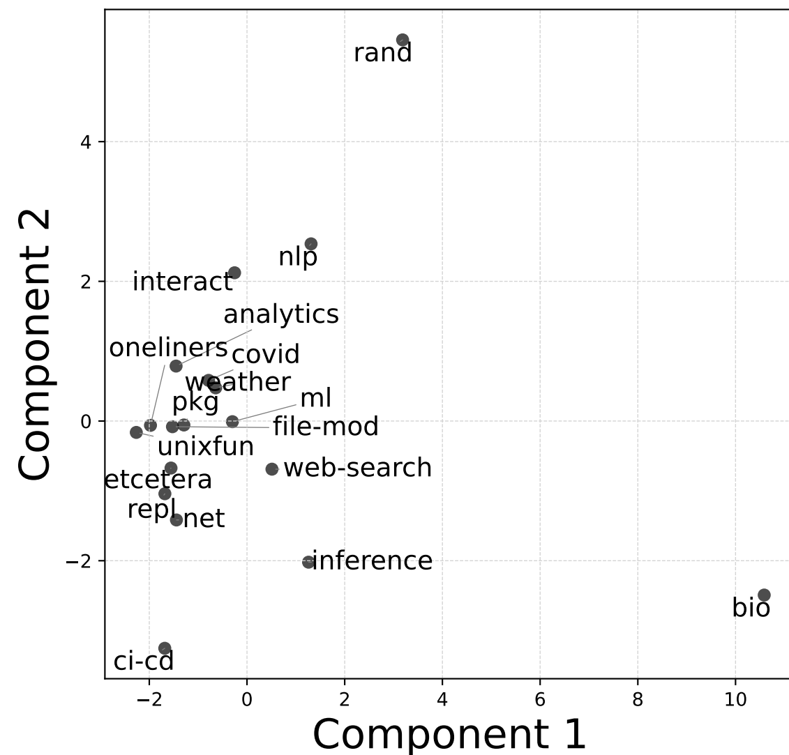
PCA from language model embeddings
