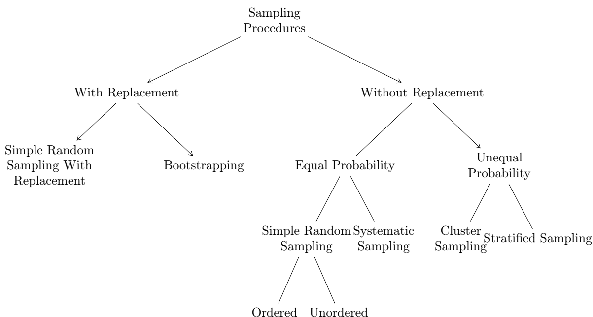
Figure 13.1: Some examples of sampling procedures, categorised by whether units are replaced or not.
