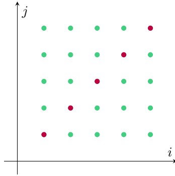
Figure 7.2: The diagonal elements correspond to when i = j . The off-diagonal entries are symmetric about i = j so their sum is equal to twice the entries strictly above (resp. strictly below) the line i = j .
