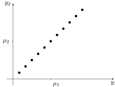
Figure 7.1: A figure of (seemingly?) dependent observations for (y_1, y_2) .
