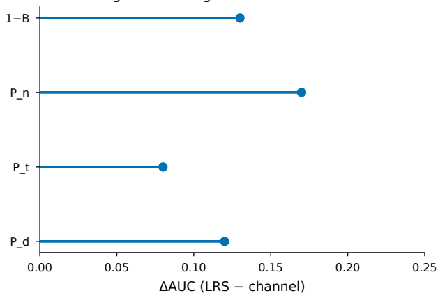
ensemble gain over single channel
