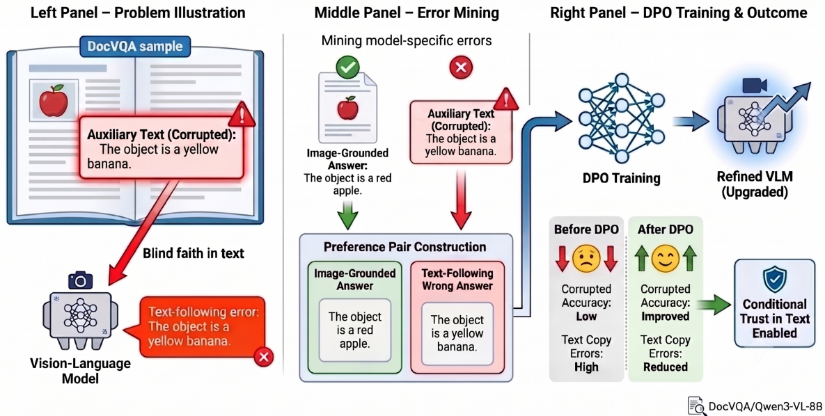
Figure 1. Overview of our mitigation. We mine cases where the base VLM follows corrupted auxiliary text, then train a DPO preference that ranks the image-grounded answer above the model’s own text-following error.
