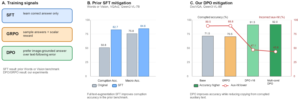
SFT and DPO reduce blind faith in text through different supervision signals
