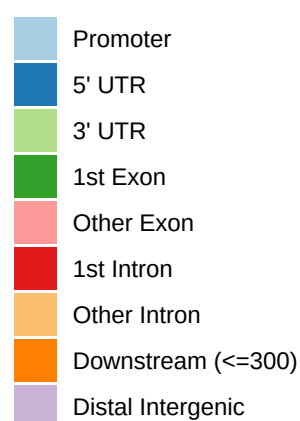
Feature
