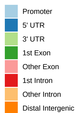
Feature
