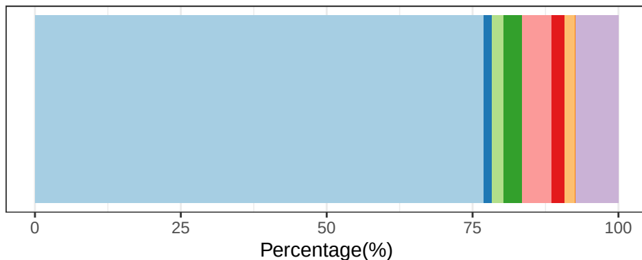
PNC – 1,274 peaks
