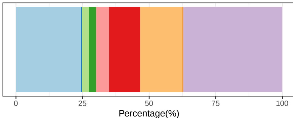
EpiLC – 5,808 peaks
