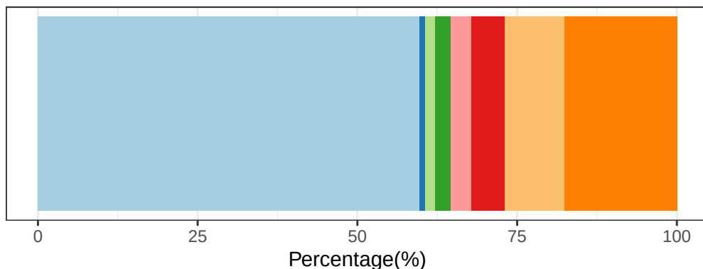
PNC – 1,274 peaks
