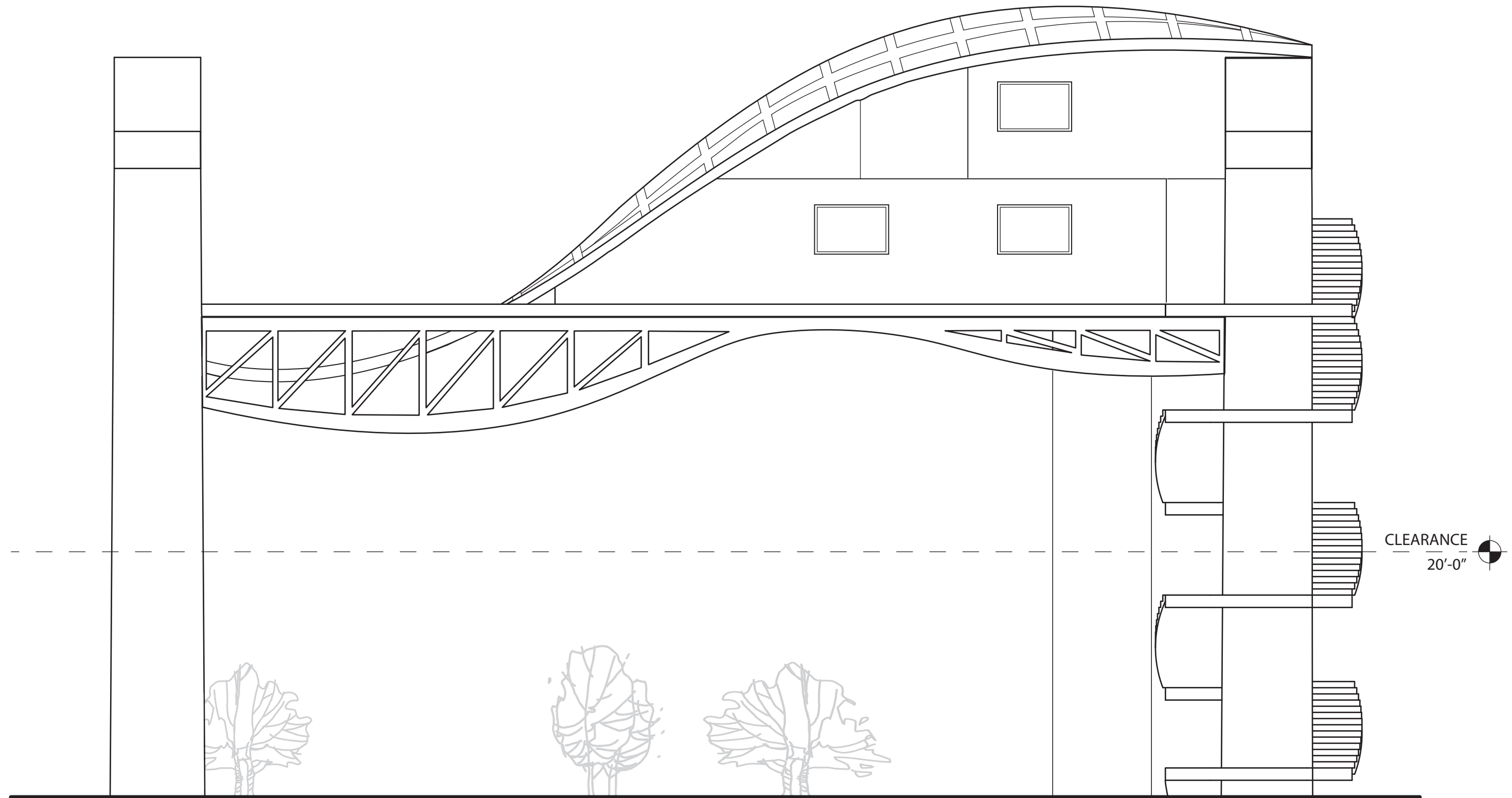
EAST ELEVATION SCALE: 1/8"=1'-0"
