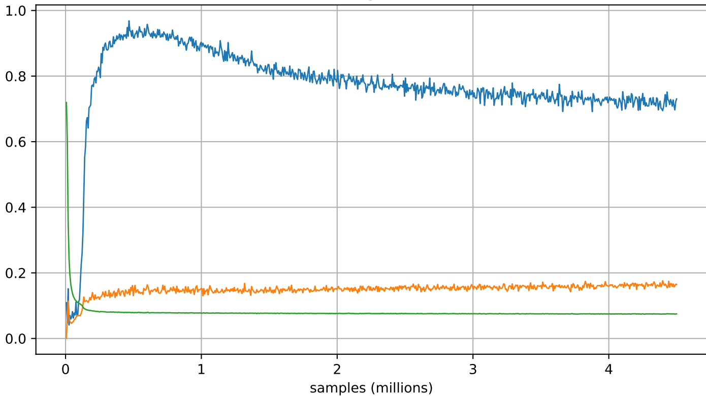
Training losses
