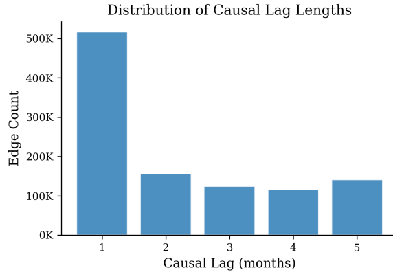
Figure 2: Distribution of optimal causal lag across all Granger and Transfer Entropy edges. Lag-1 dominates but longer lags contribute meaningful structure.
