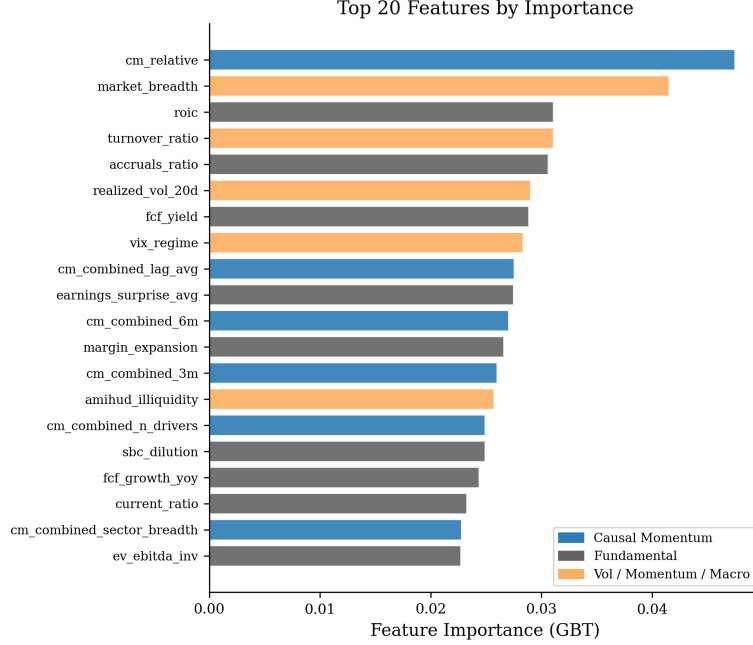
Figure 8: Top 20 features by GBT importance. Blue bars indicate causal momentum features; gray bars are fundamentals; orange bars are volatility/momentum/macro. The top feature is cm_relative .
