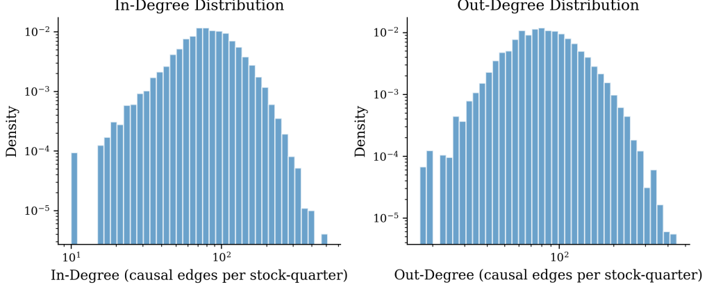
Figure 3: In-degree and out-degree distributions of the causal graph (log-log scale). Heavy tails suggest scale-free properties.
