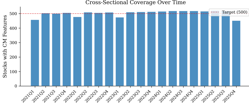
Figure 6: Number of stocks with causal momentum features per quarter. Coverage exceeds 90% of the universe in all complete quarters.
