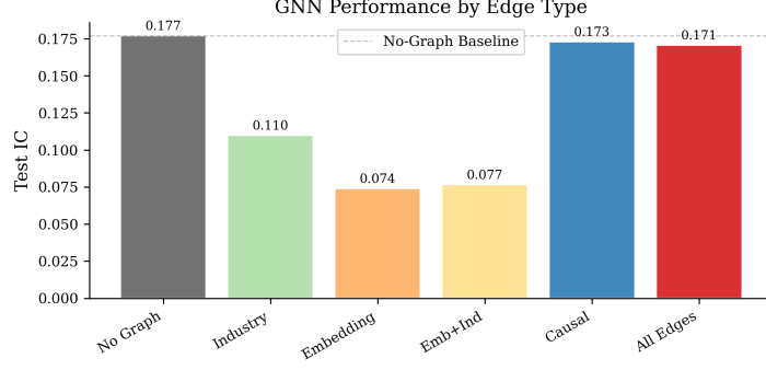
Figure 9: GNN test IC by edge type. Causal edges are the only type that allows the GNN to approach (but not exceed) the no-graph baseline.
