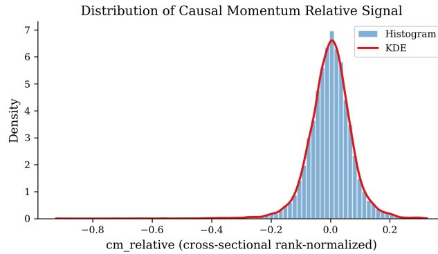
Figure 5: Distribution of cm_relative with kernel density estimate. The feature is approximately symmetric and well-behaved after cross-sectional rank normalization.
