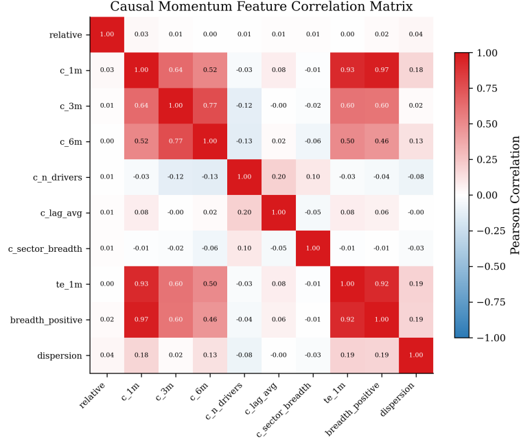
Figure 4: Correlation matrix of the 10 retained causal momentum features. Combined/Granger variants are highly correlated; cross-sectional features ( cm_relative , cm_dispersion ) offer orthogonal signal.
