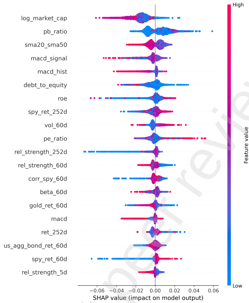
Figure 7: SHAP Summary
