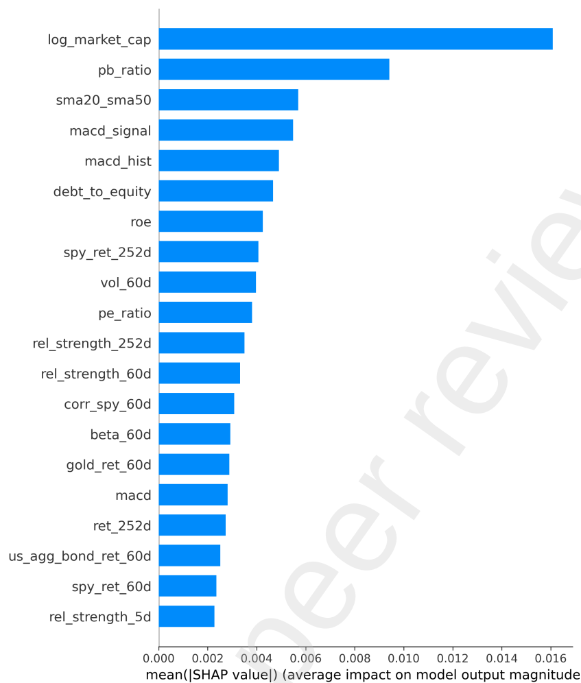
Figure 6: SHAP Importance
