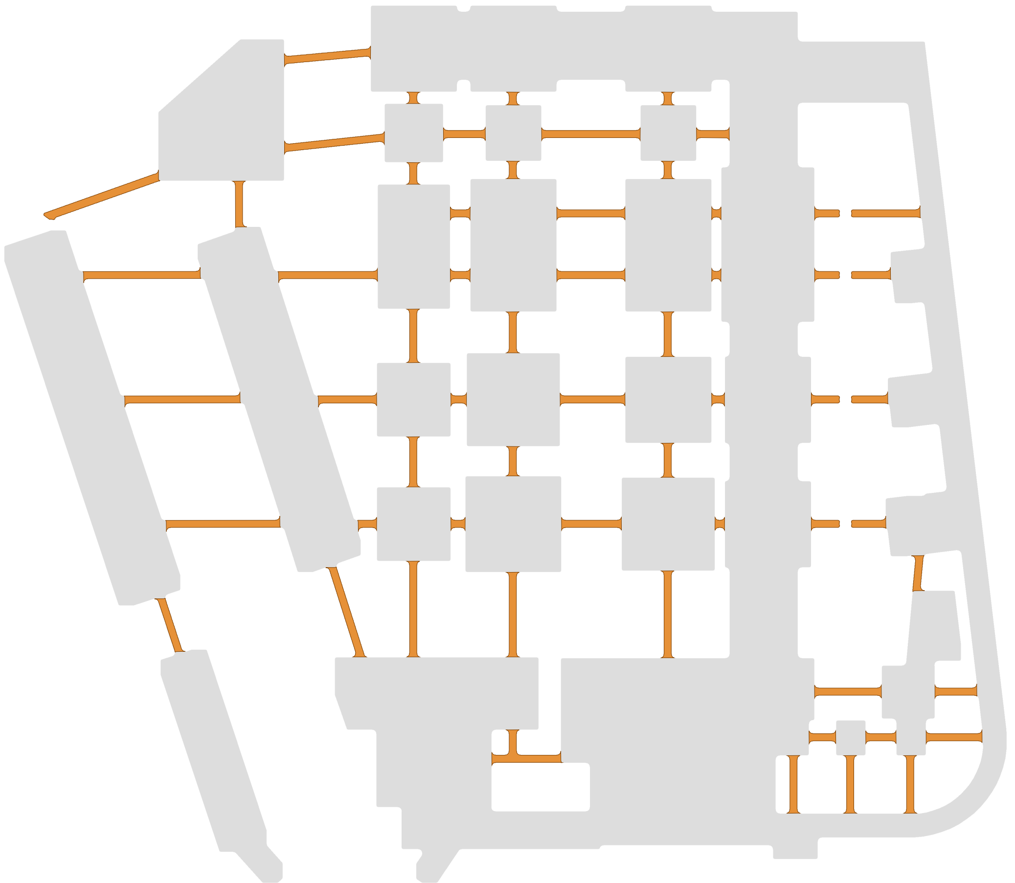
Blinding under ground beams only — 100 mm each side — 117.24 m 2
