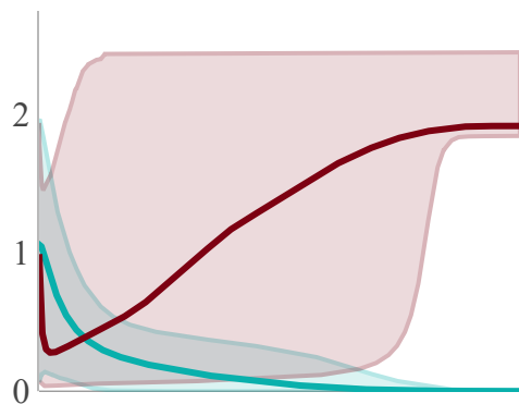
E. Intervention on Motivation Rate
