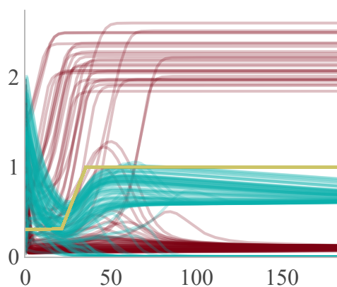
E. Intervention on Motivation Rate
