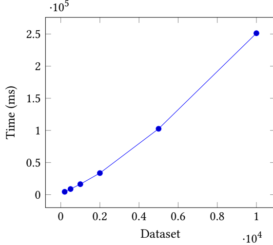
Figure 3: Plot of execution time corresponding to the dataset. Data shown in 2. This plot reinforces the claim that NN-Descent has a complexity of O(n^{1.14}) due to its shape.
