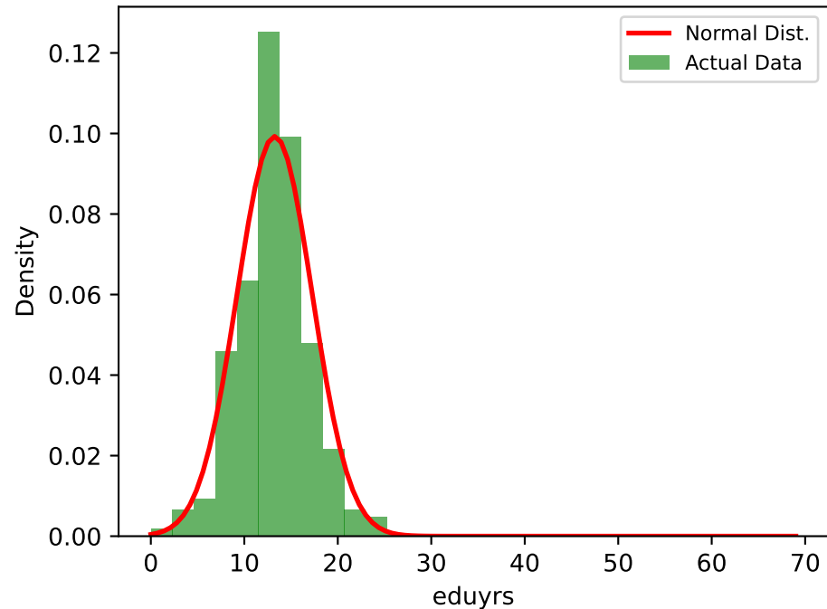
Feature: eduyrs
