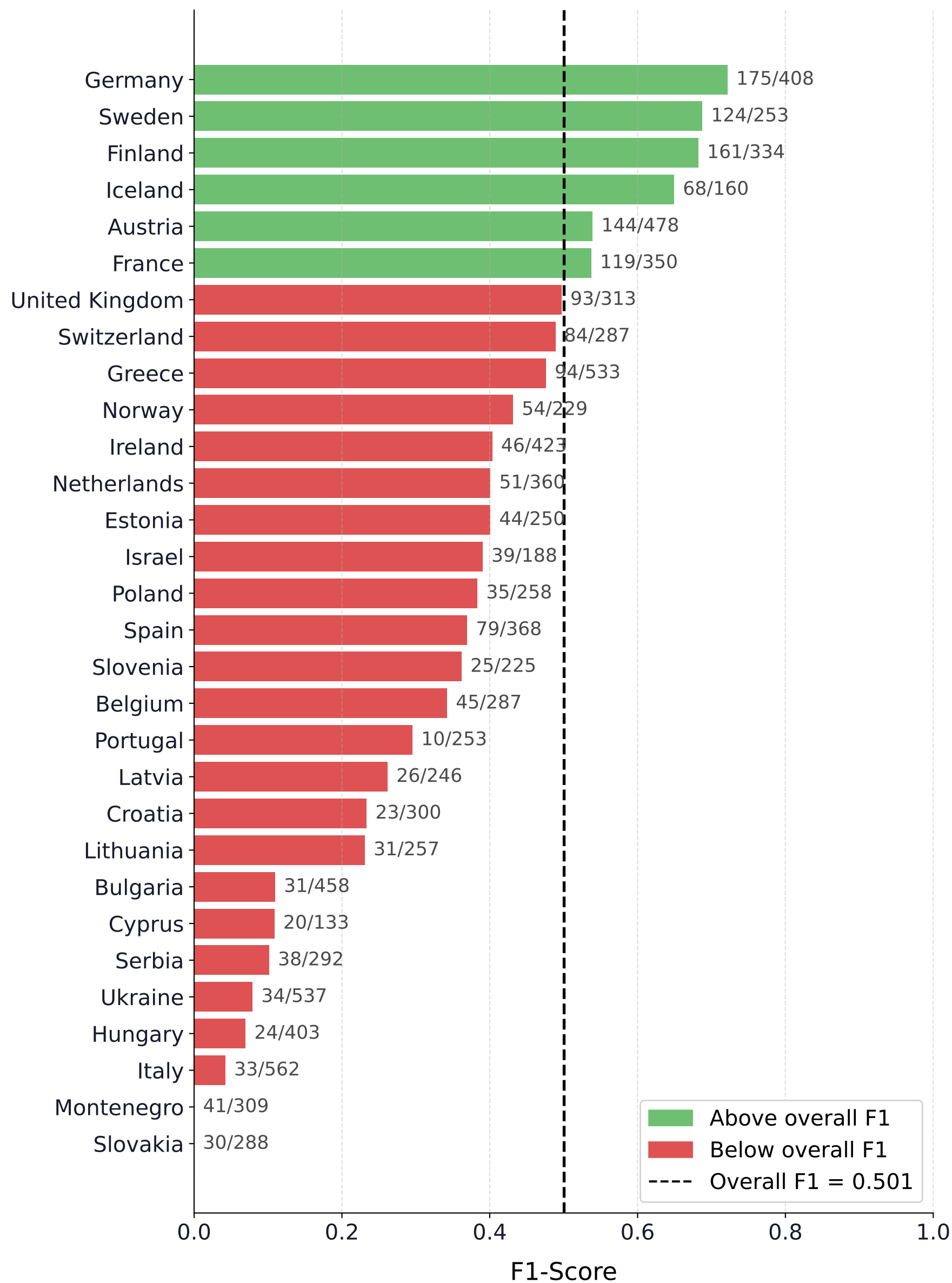
F1-Score by Country
