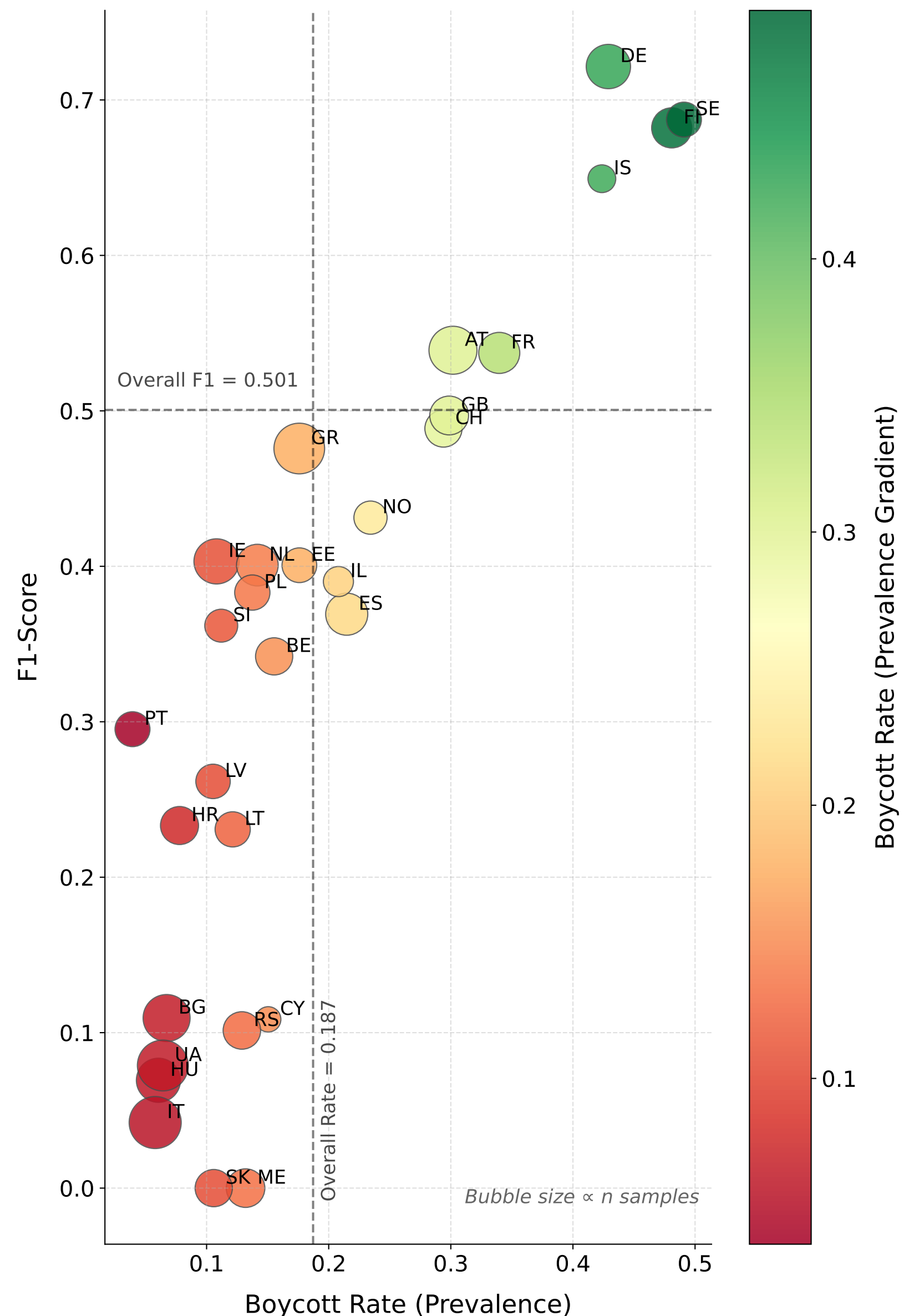
Boycott Prevalence vs F1 (bubble size = n samples)
