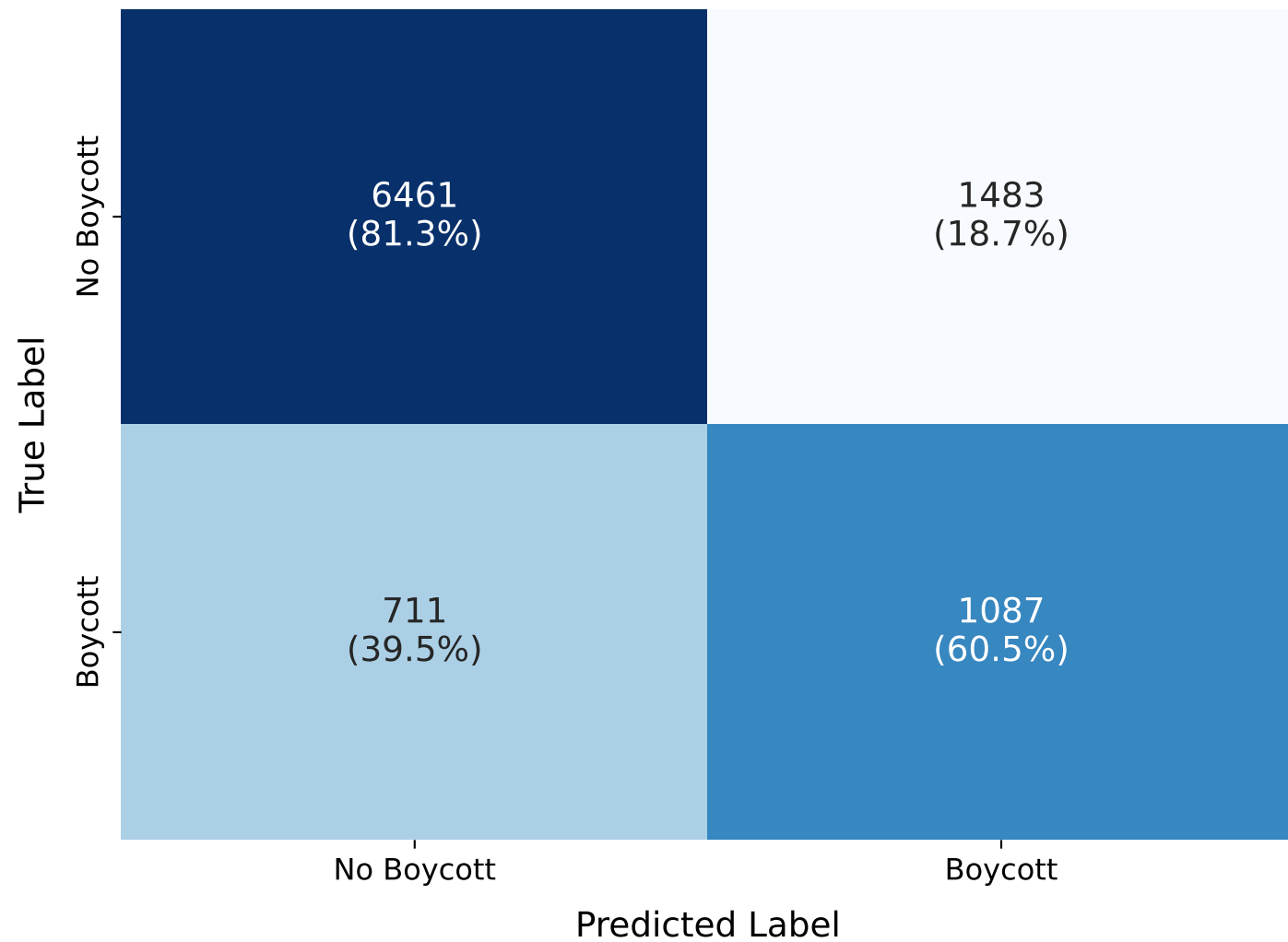
Recall-Normalized Confusion Matrix
