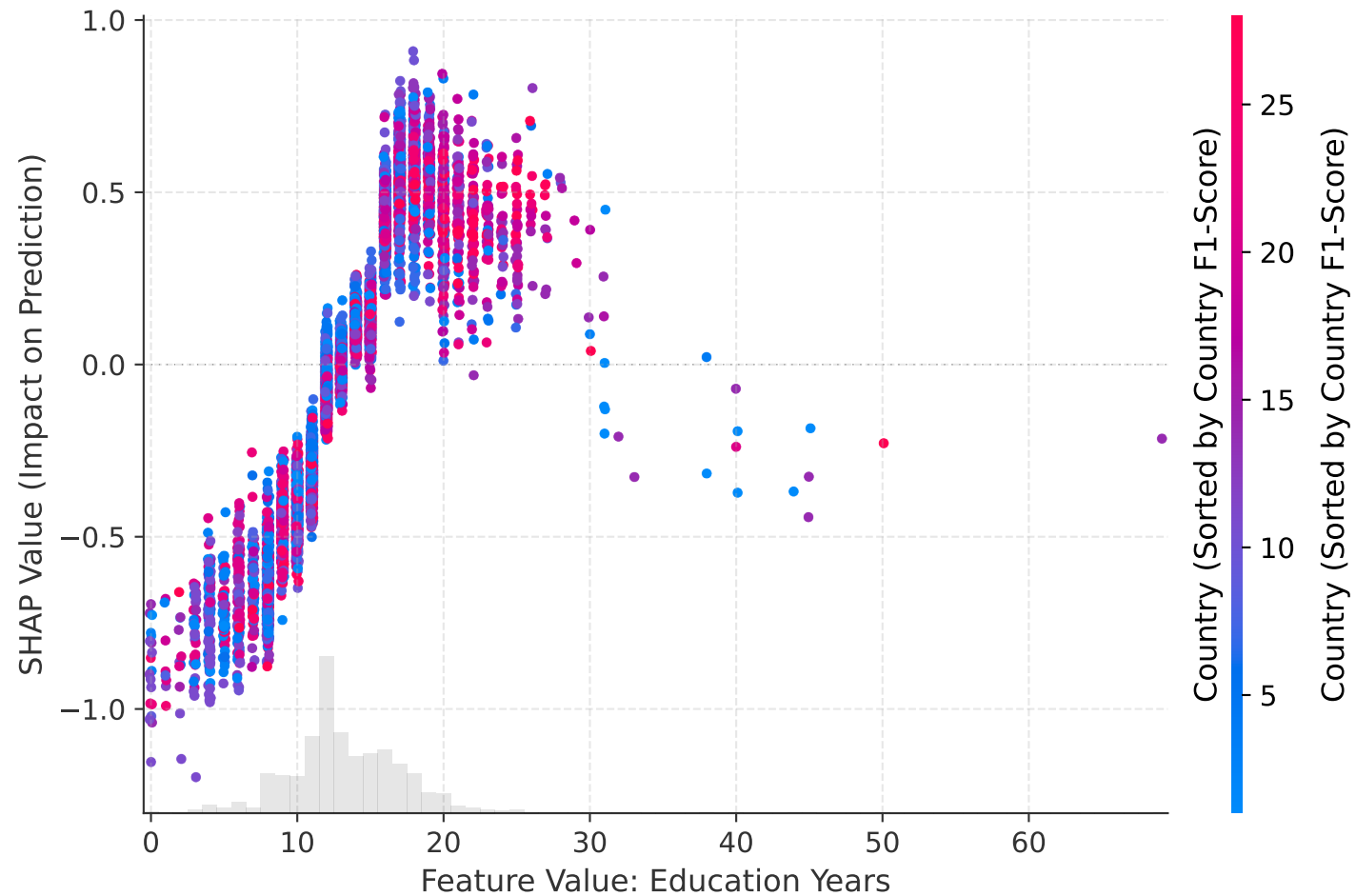
SHAP Dependence Plot: Education Years
