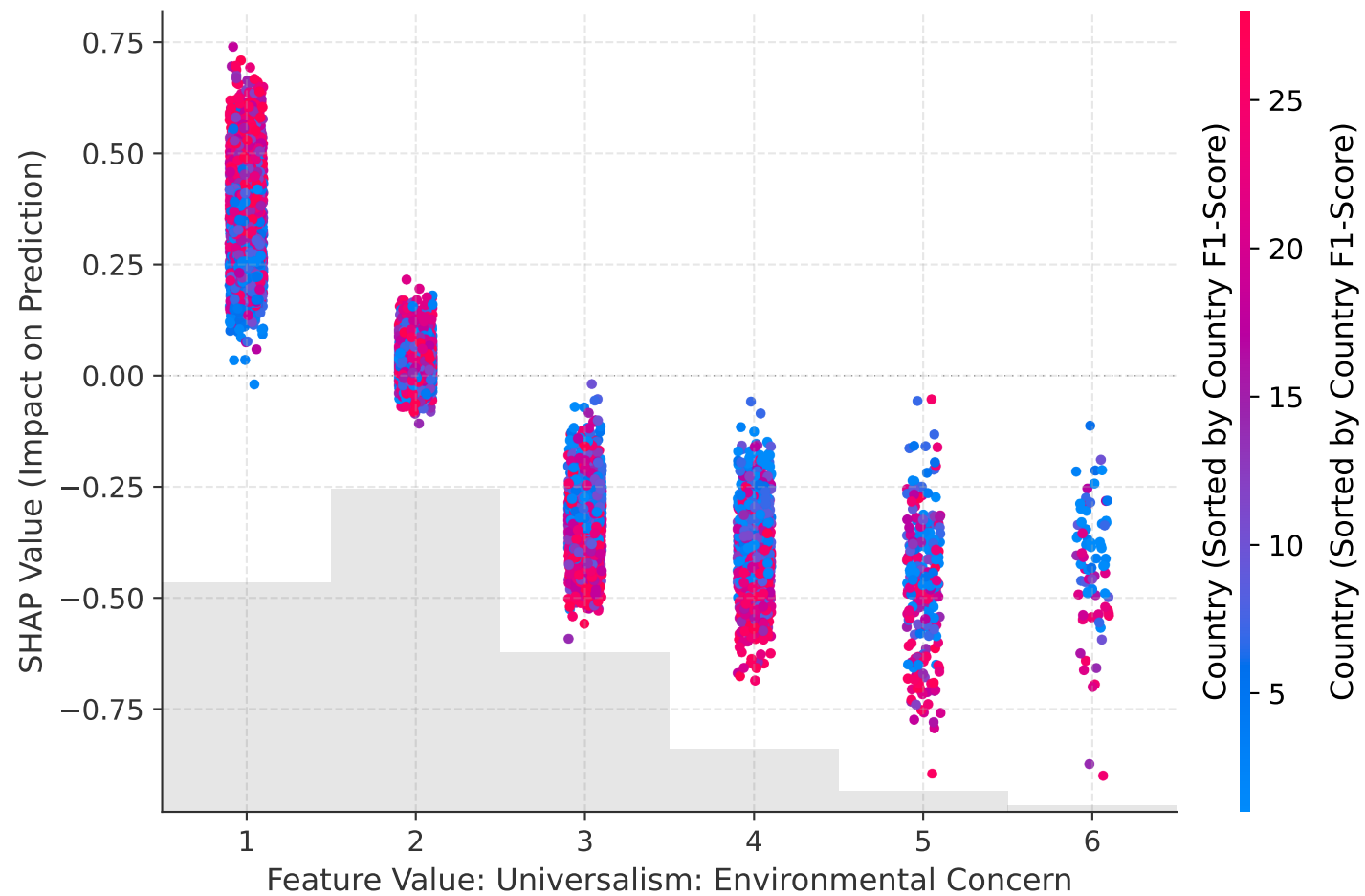
SHAP Dependence Plot: Universalism: Environmental Concern
