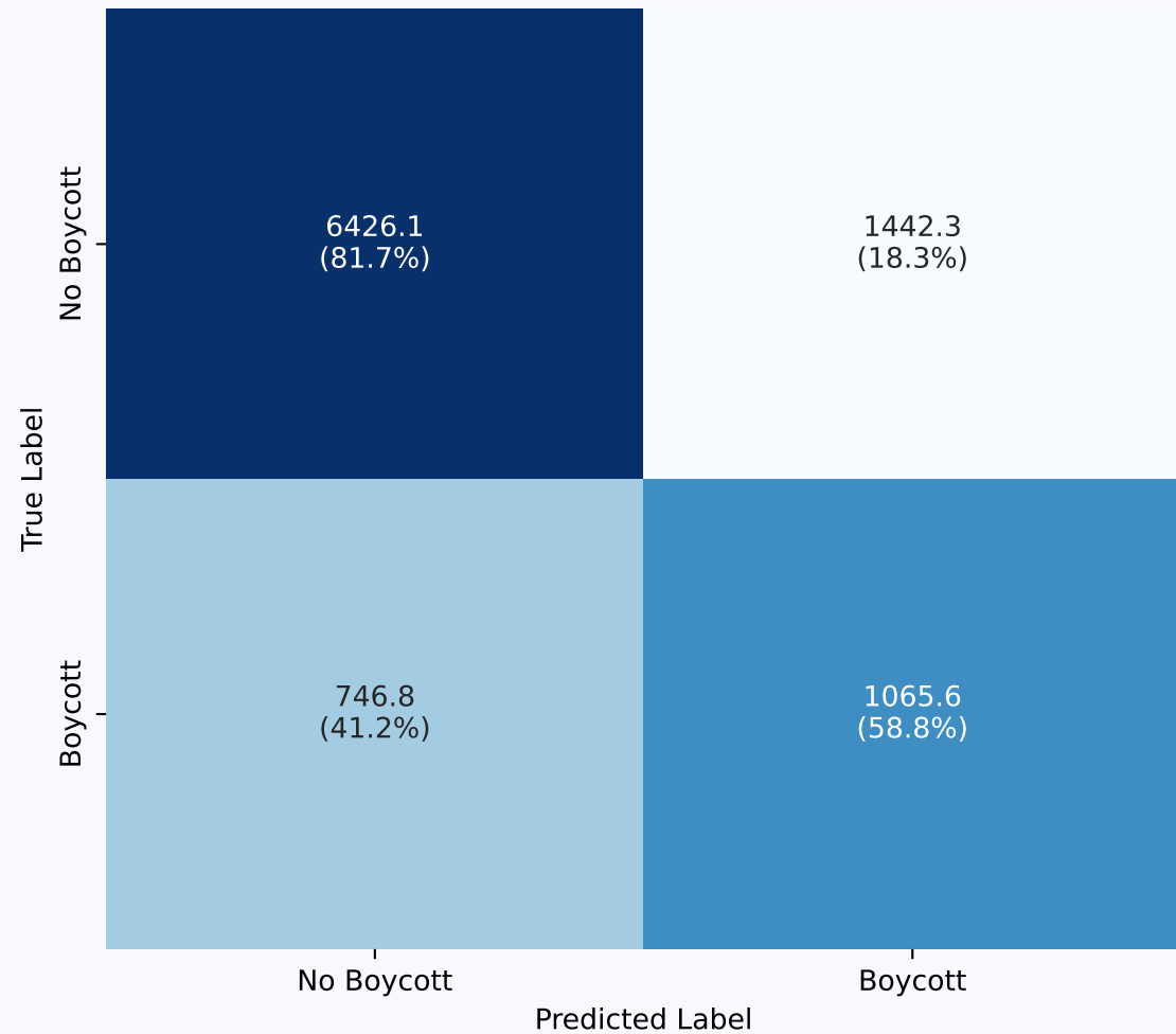
Weighted Confusion Matrix (Class-weighted CatBoost)
