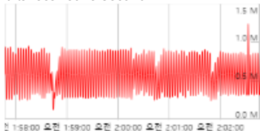
bitsReceivedPerSecond
