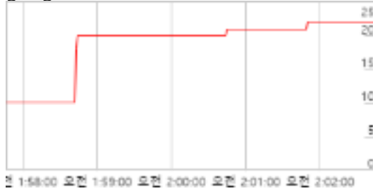
googRenderDelayMs
