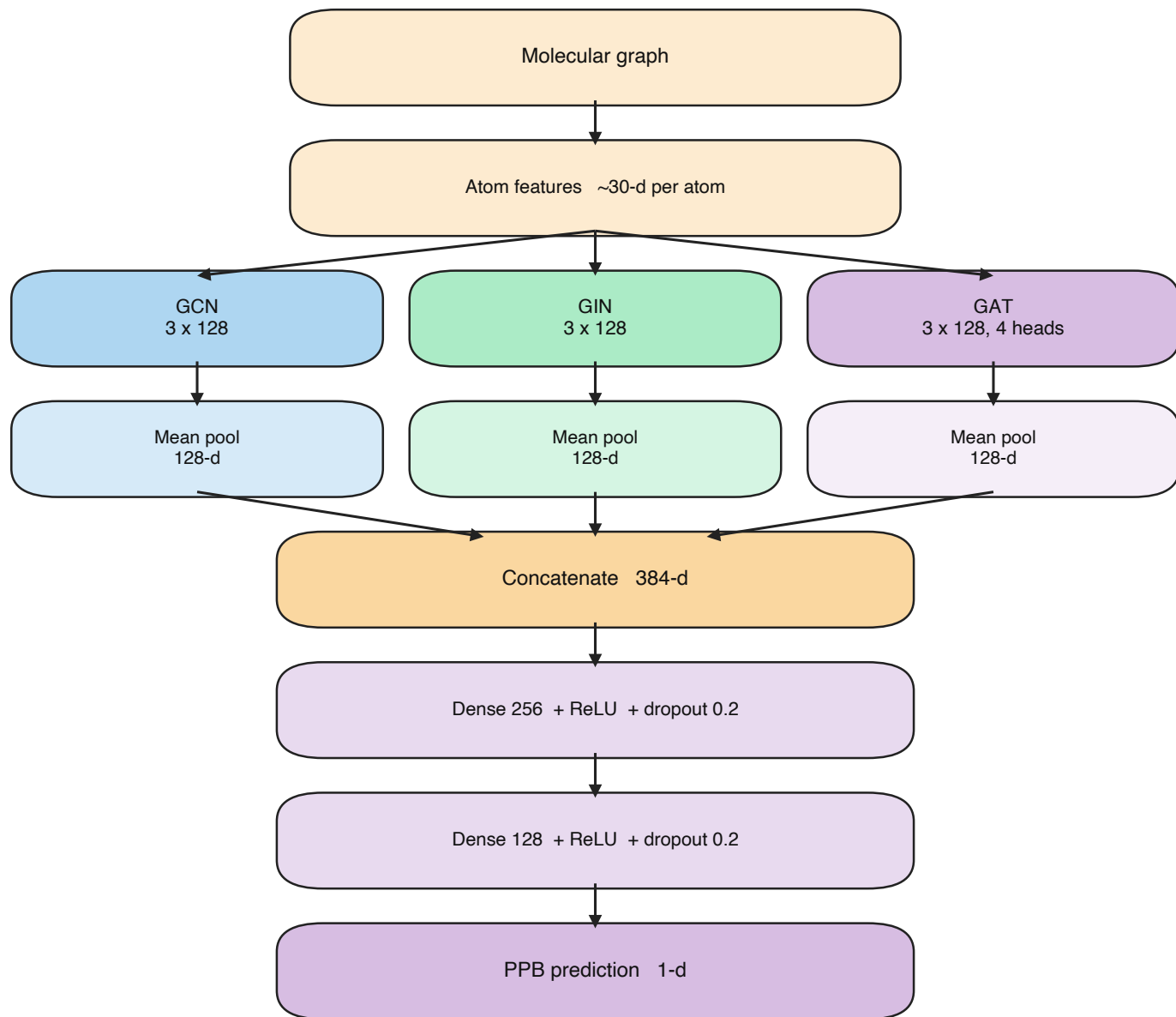
Supplementary Figure 3. GCN+GIN+GAT. No ChemBERTa. Graph stacks match the standalone GCN, GIN, and GAT. ~0.35M parameters.
