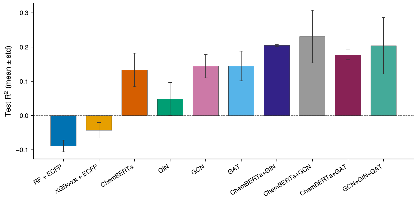
PPB test R^2 under one Bemis--Murcko scaffold split
