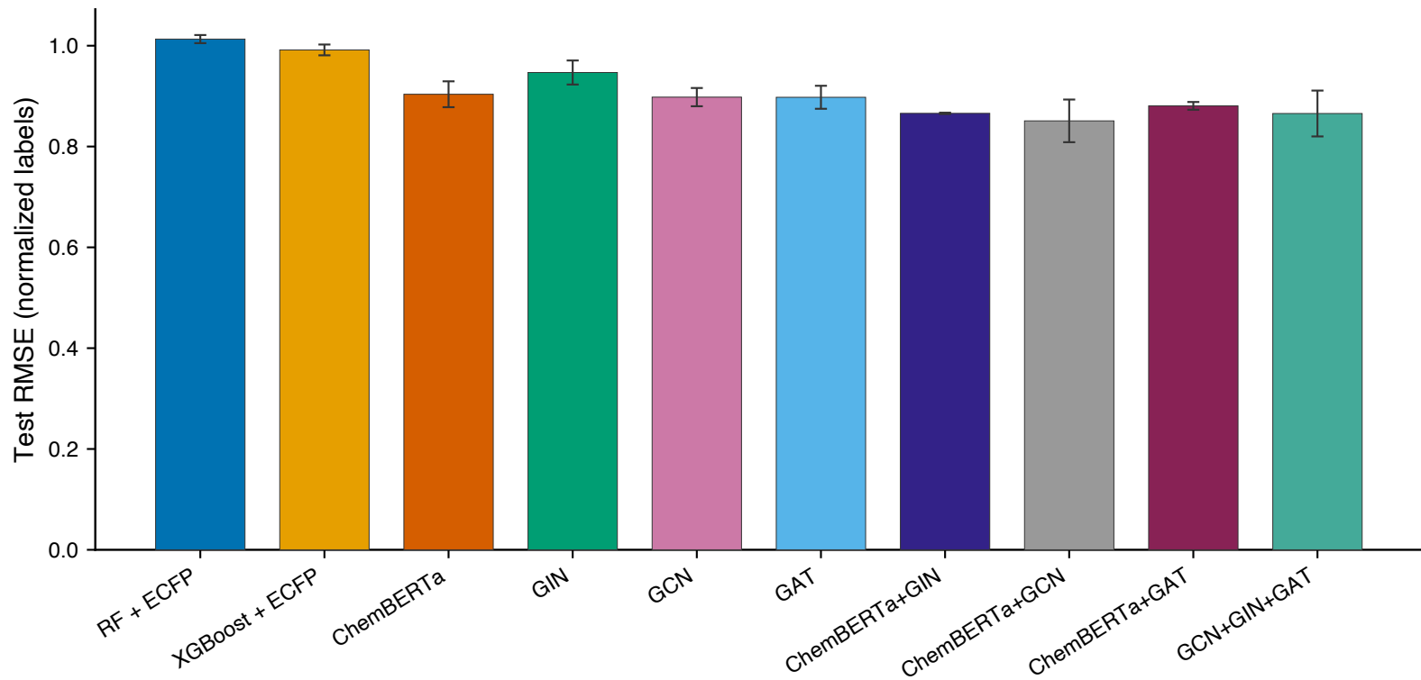
PPB test RMSE under one Bemis--Murcko scaffold split
