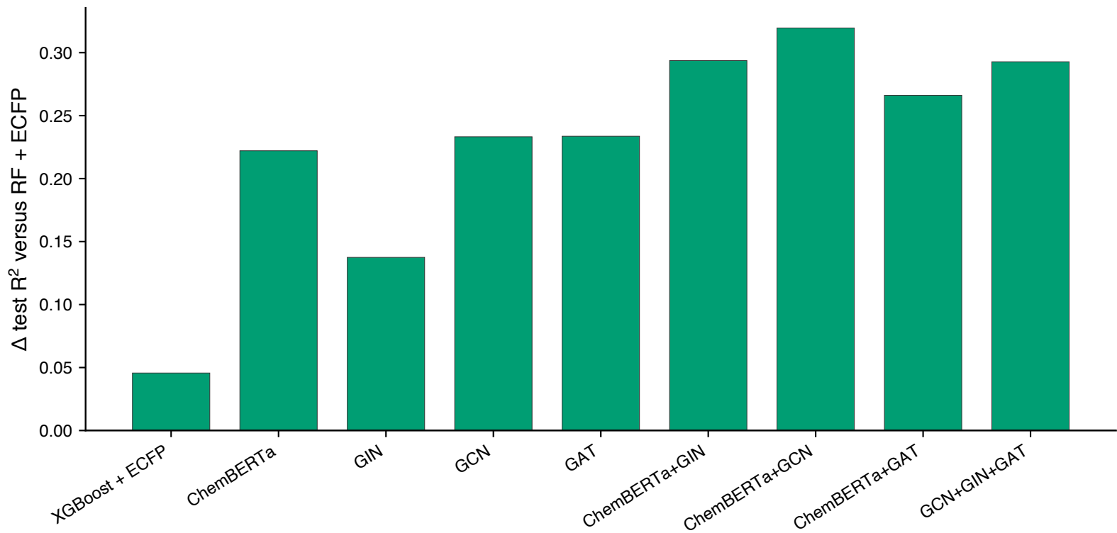
Mean test R^2 relative to random forest
