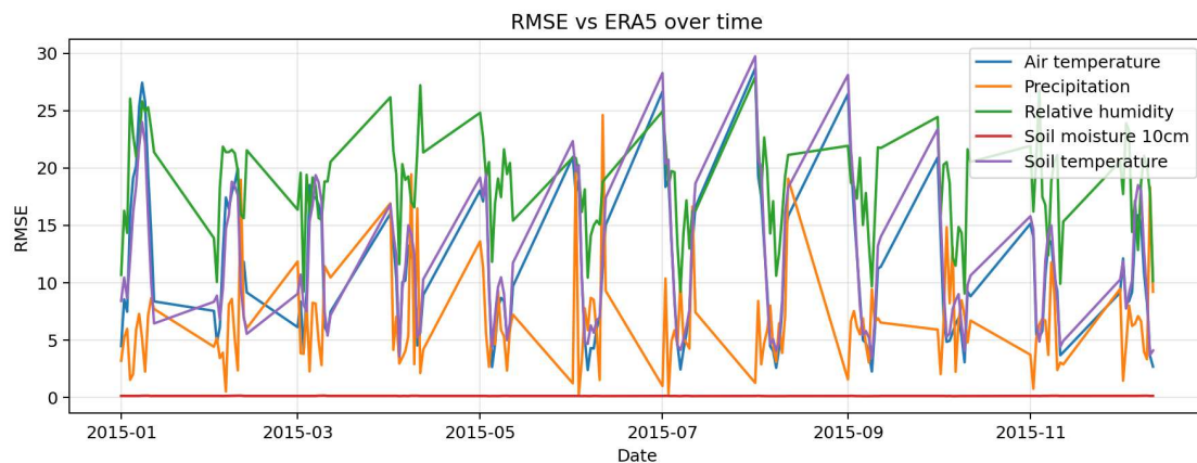
RMSE variation over time for different variables
