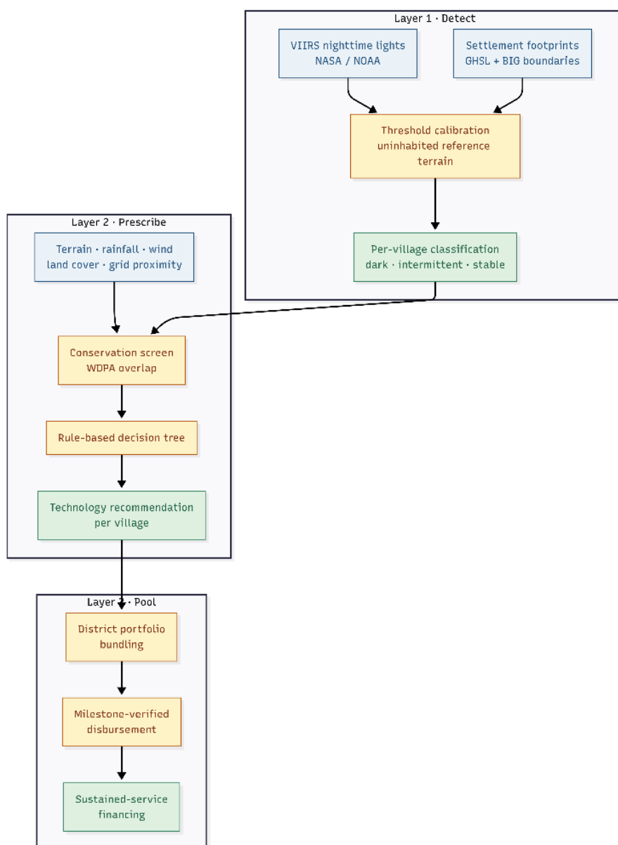
Figure 3. Terang three-layer architecture: Detect, Prescribe, Pool, showing the data inputs to each layer and the outputs passed downstream. The verification and disbursement stages shown in the diagram are described under Future Possibilities as the next operational extension.
