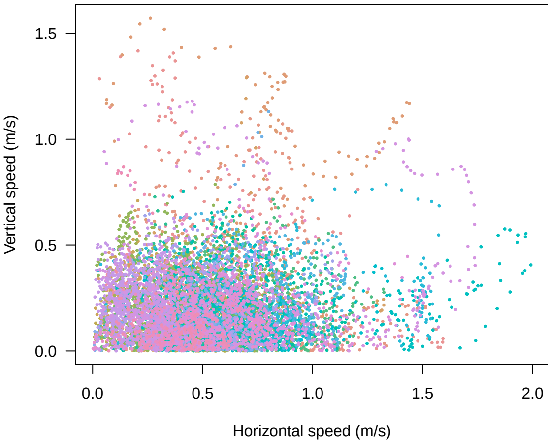
Flight speed distribution (real data)
