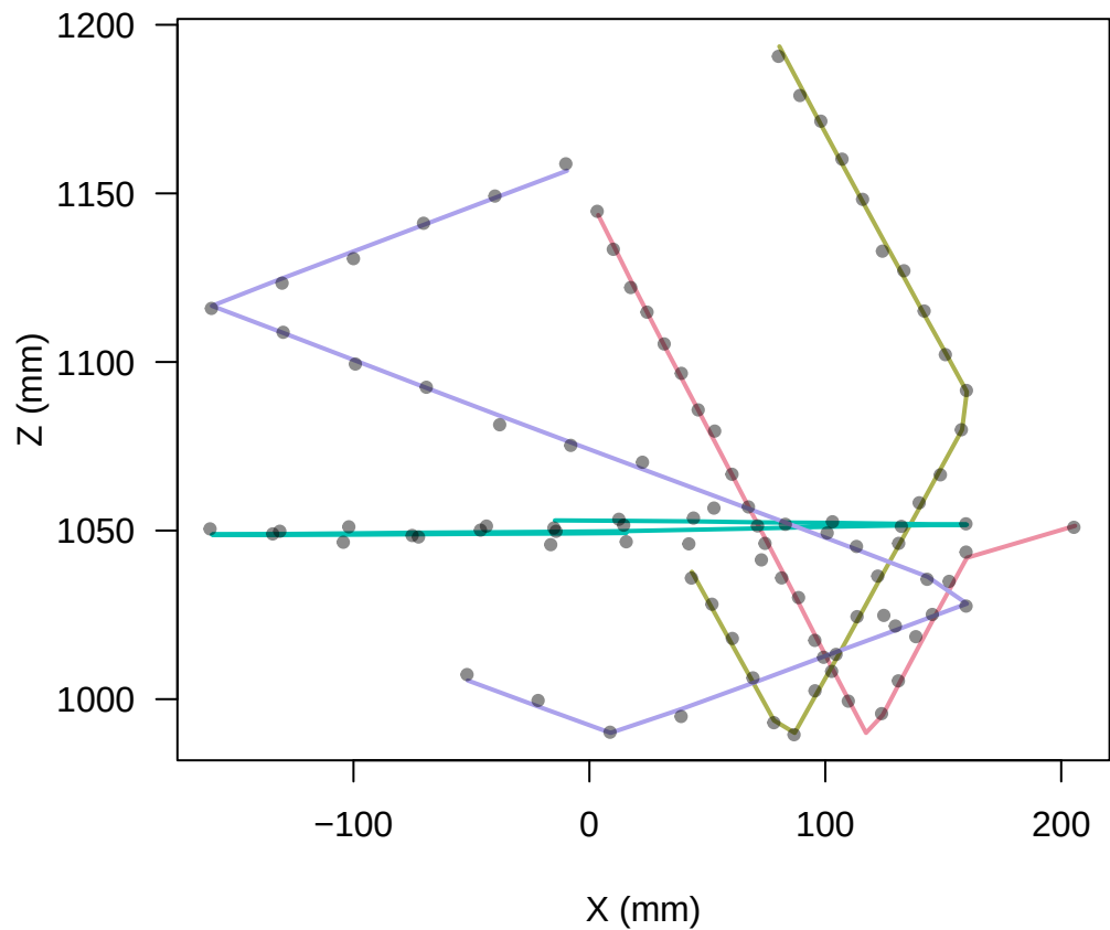
X-Z plane: true paths (lines) vs recovered (points)
