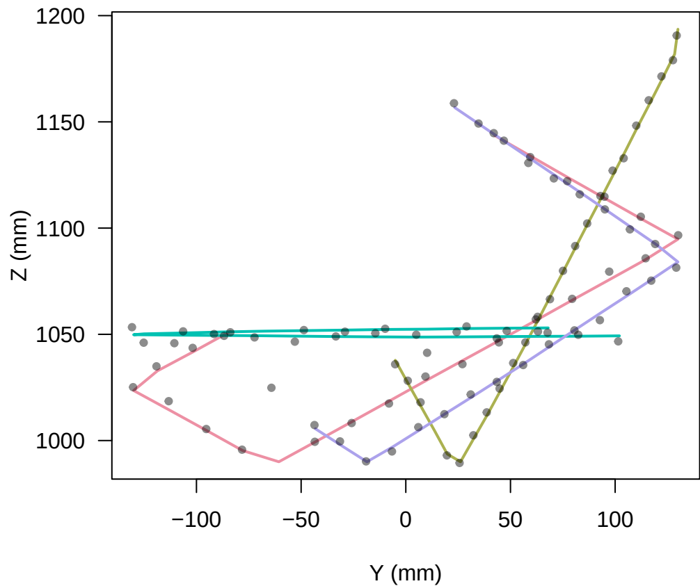
Y-Z plane: true paths (lines) vs recovered (points)
