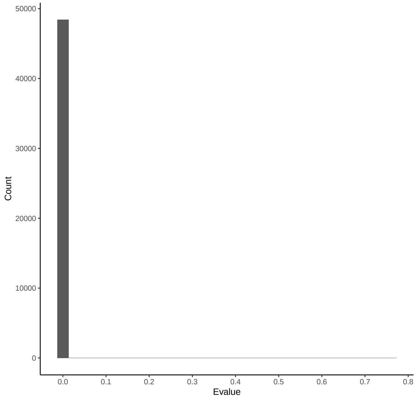
Evalue frequencies (n=48431 BLAST hits)
