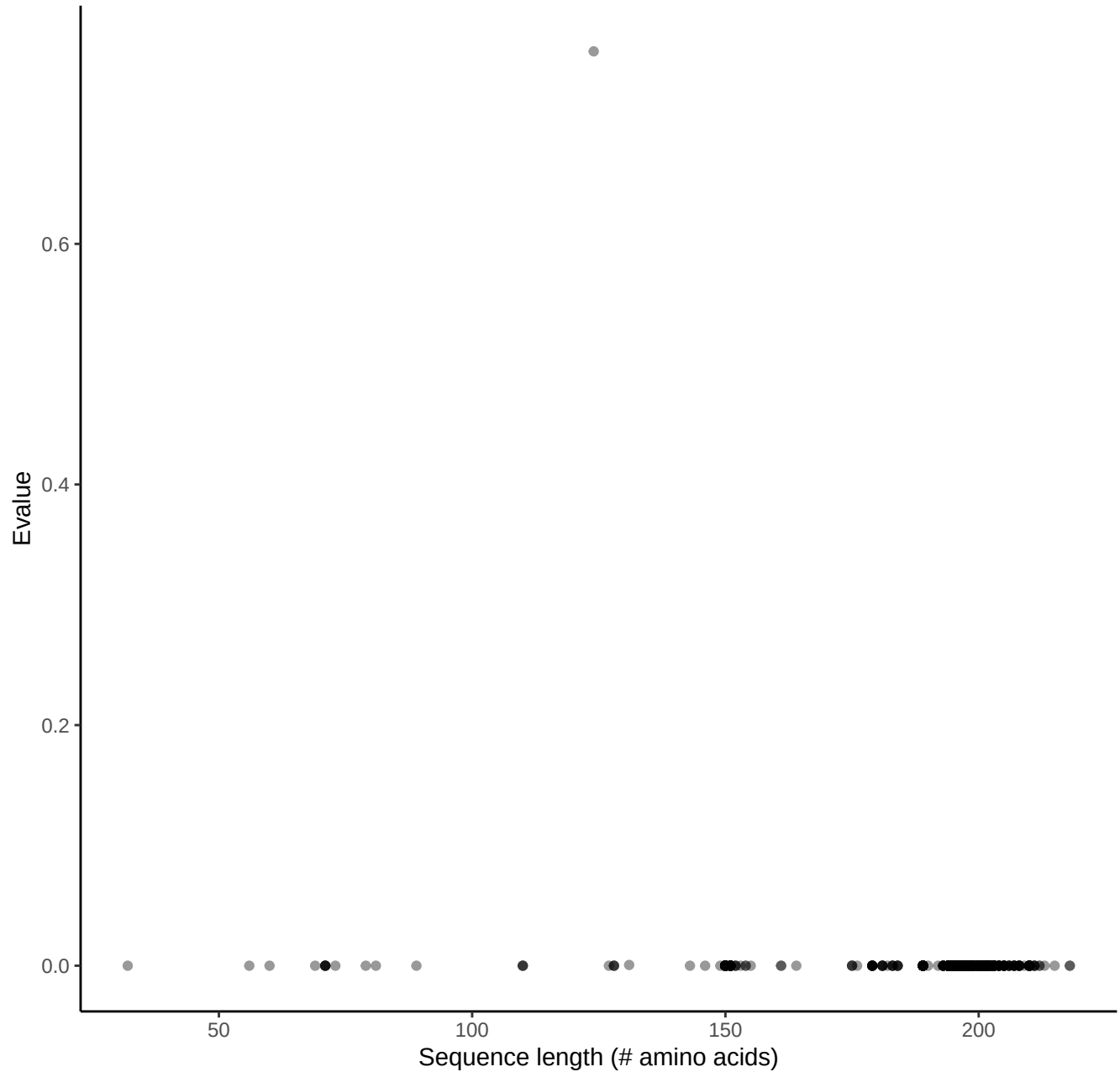
Sequence length vs evalute plot (n=48431 BLAST hits)
