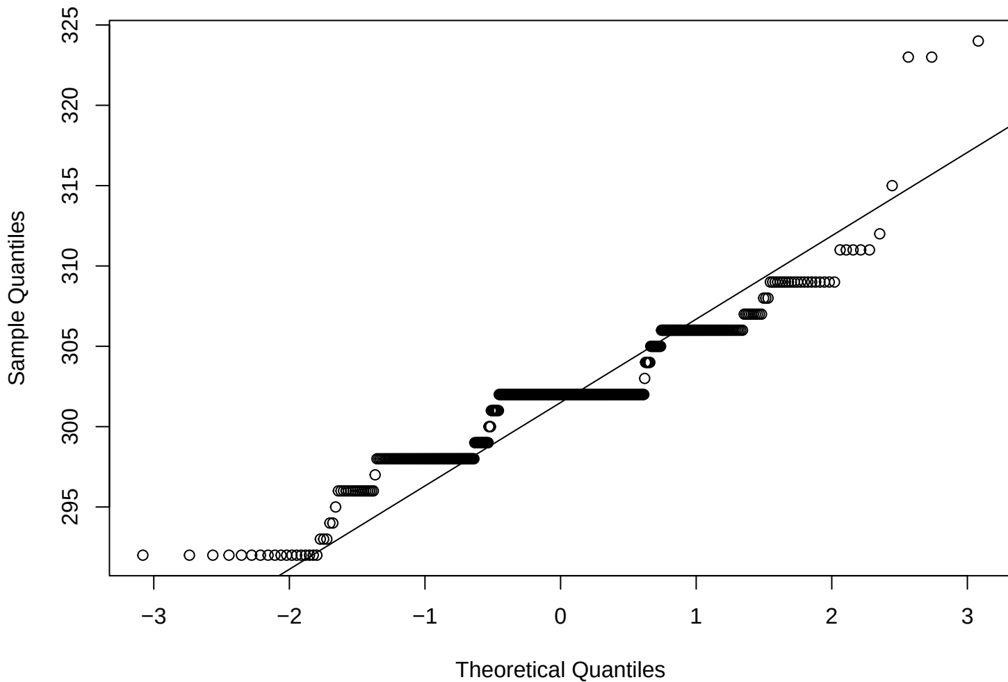
QQ Plot of sequence_length
