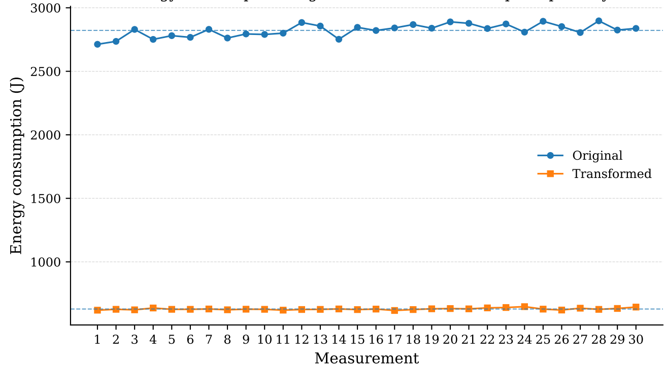
Energy Consumption original vs transformed: sample repository
