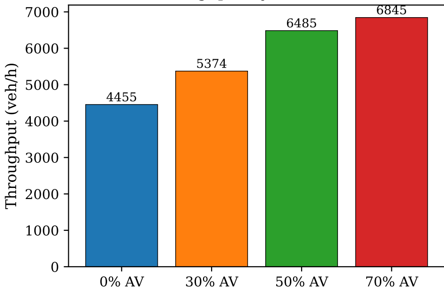
Network Throughput by AV Penetration Rate
