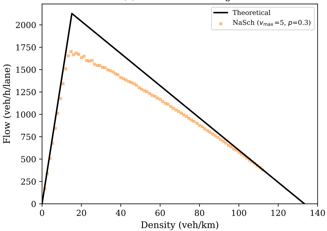
(c) NaSch — full range
