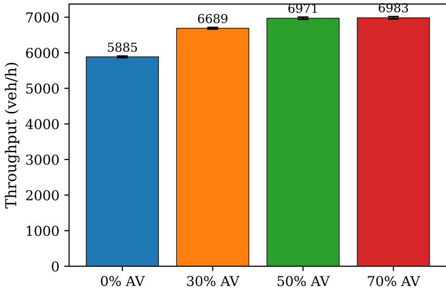
Network Throughput by AV Penetration Rate (mean \pm 95% CI, N=20)
