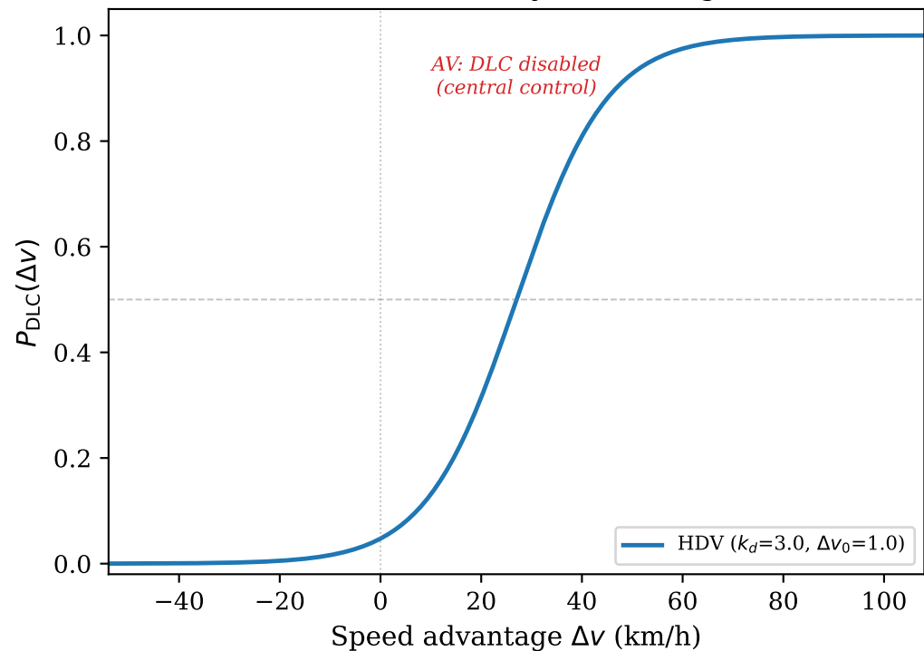
(b) Discretionary lane change
