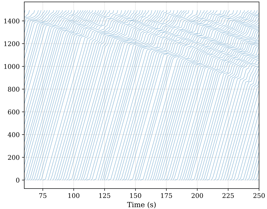
(b) Congested (2400 veh/h)
