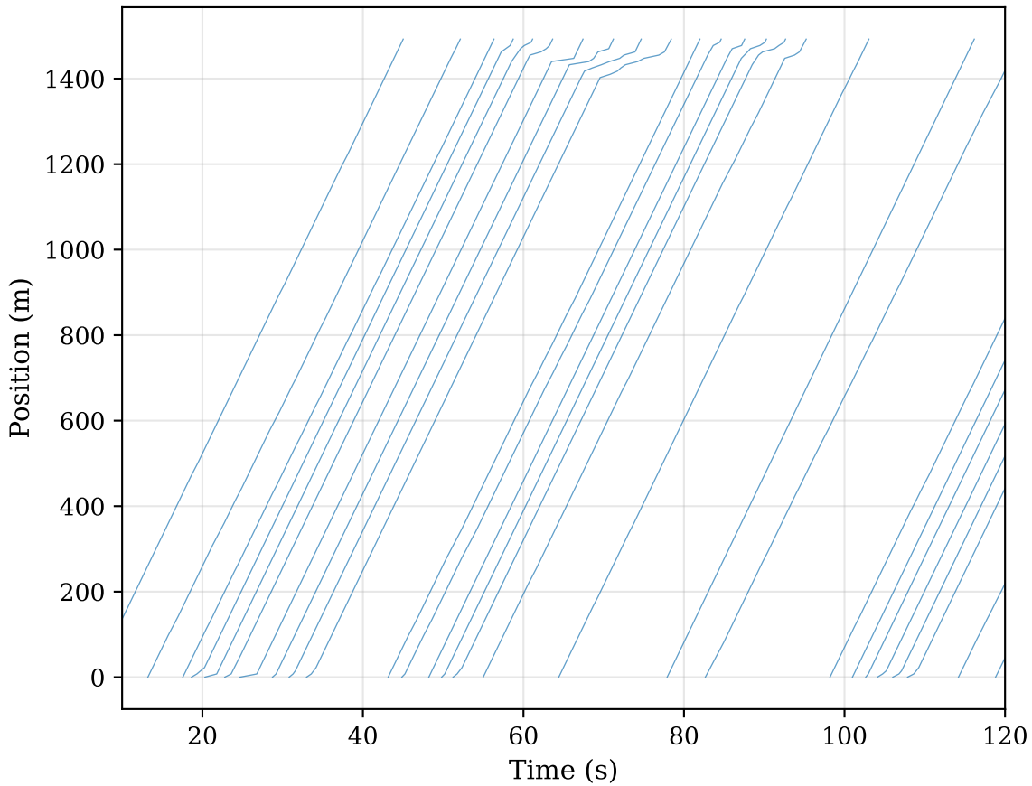
(a) Free-flow (800 veh/h)
