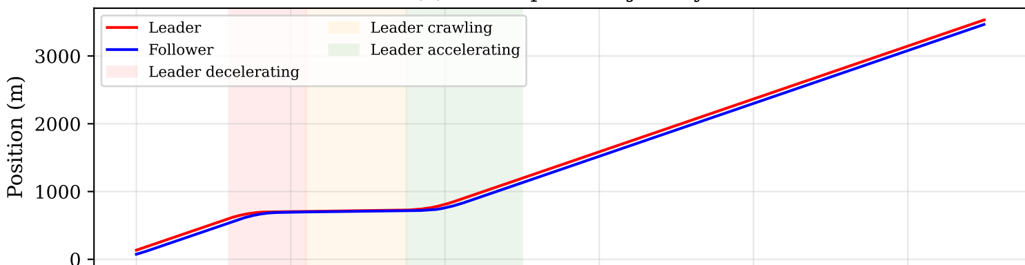
(a) Time-Space Trajectory
