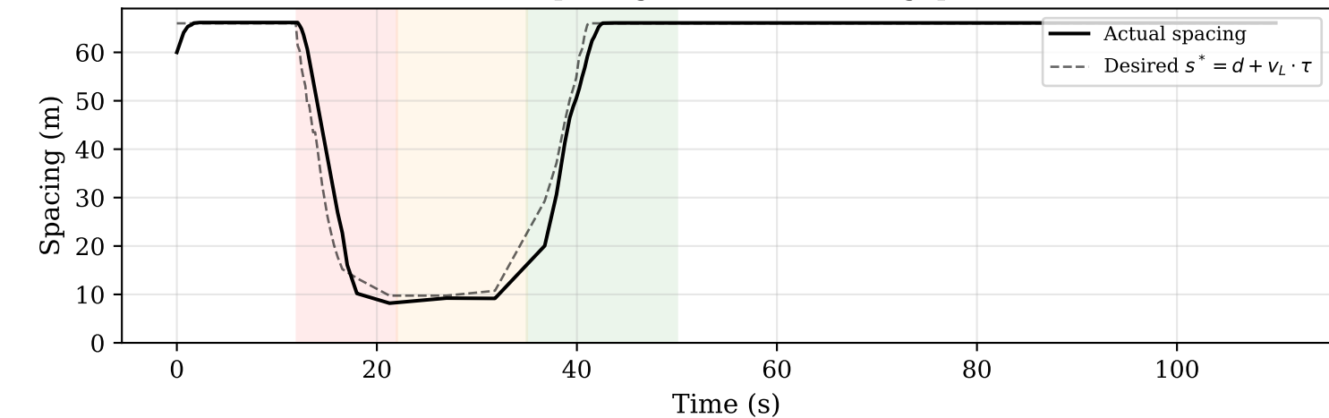
(c) Spacing (leader-follower gap)
