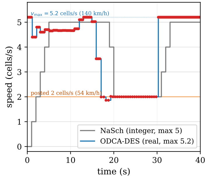
(c) speed of the last vehicle: up, down at the zone, up again
