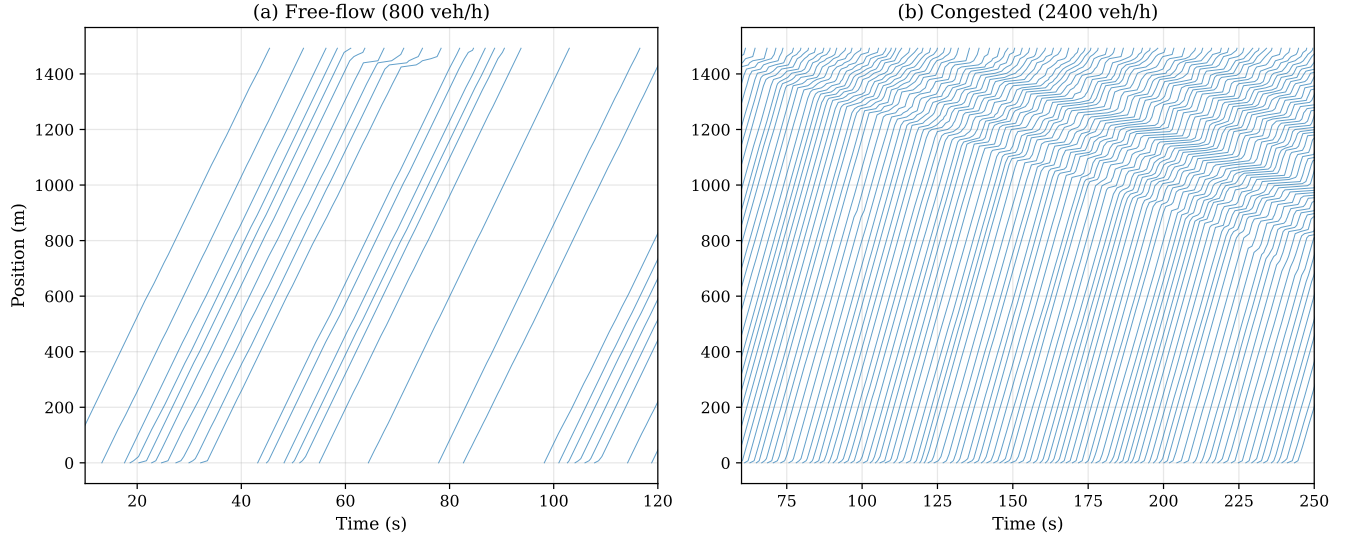
Figure 6: Time-space diagrams on a single-lane segment. (a) Free-flow (800 veh/h): trajectories are near-parallel with slope v_f = 5.2 cells/s ( \approx 140 km/h), with minor perturbations from HDV random slowdowns. (b) Congested (2400 veh/h): trajectory slopes decrease as density exceeds capacity, with backward-propagating waves visible as slope transitions. Trajectories are coloured by each vehicle's average speed (blue above 100 km/h, orange 40–100, red below 40); at this demand every vehicle averages above 100 km/h, and the congestion shows as the bending of individual trajectories rather than as slow vehicles. The disturbances visible in panel (b) travel upstream, the direction the theory gives for w = \ell/\tau = 0.667 cells/s ( \approx 18 km/h).
