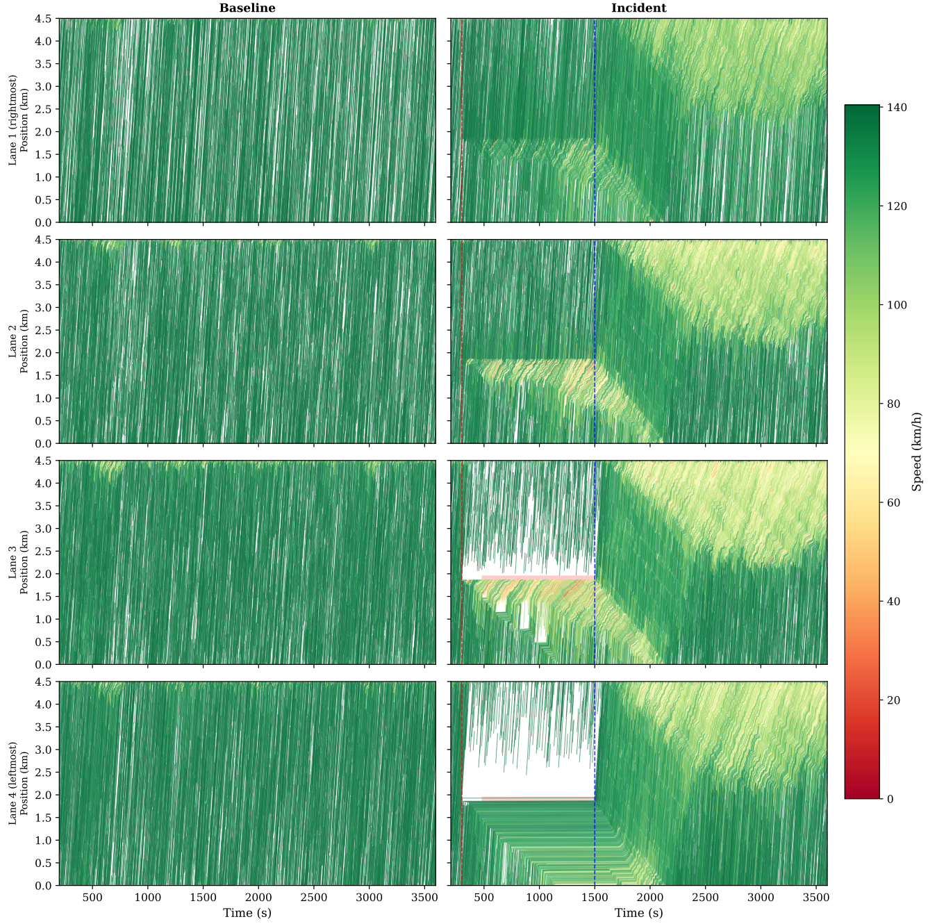
Figure 13: Lane-by-lane time-space diagrams: baseline (left) vs. the 20-minute closure of lanes 3 and 4 (right), at 4,500 veh/h. Trajectories are coloured by speed (green = free flow, red = stopped). Dashed lines on the incident panels mark onset ( t = 300 s, red) and clearance ( t = 1500 s, blue), and the shaded band marks the blocked cells. The baseline is free-flowing throughout; the incident panels show the blocked lanes emptying downstream, the queue growing upstream in all four lanes, and the recovery spreading upstream after clearance.
