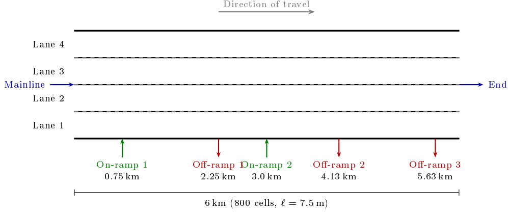
Figure 4: Test network geometry: 4-lane unidirectional freeway segment (6 km, 800 cells at \ell = 7.5 m). On-ramps merge into lane 1 (rightmost); off-ramps exit from lane 1. Mainline demand enters at the first cell of each lane; traffic bound for the segment end is spread over the four lane ends (cell 800), so it crosses lanes in both directions.
