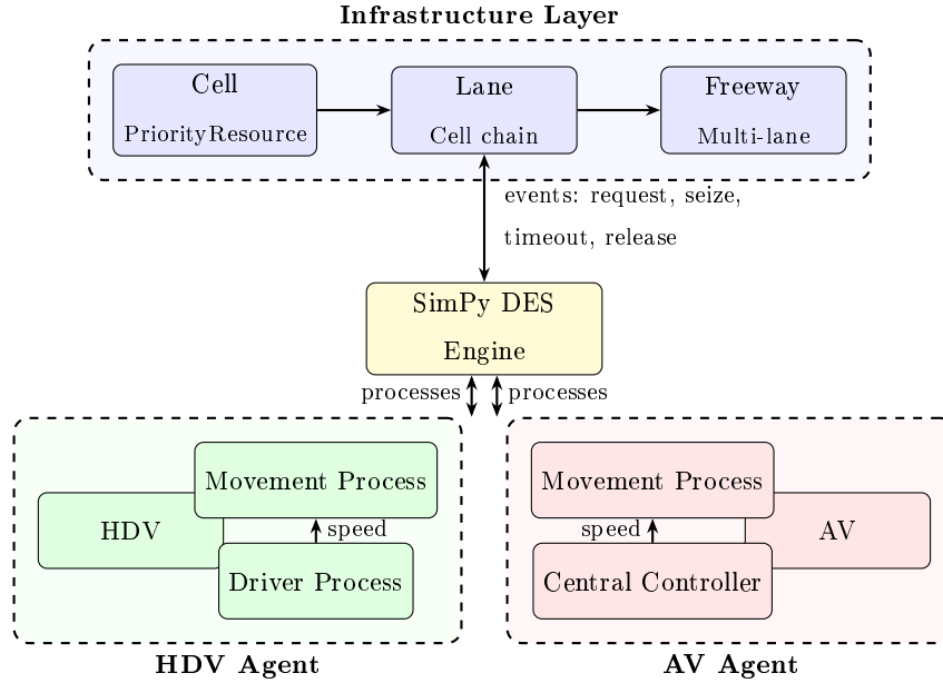
Figure 2: ODCA-DES framework architecture. Infrastructure objects provide the spatial resource structure; the DES engine manages event scheduling and process synchronization. HDVs encapsulate concurrent movement and driver processes, while AVs delegate behavioral decisions to a central controller.
