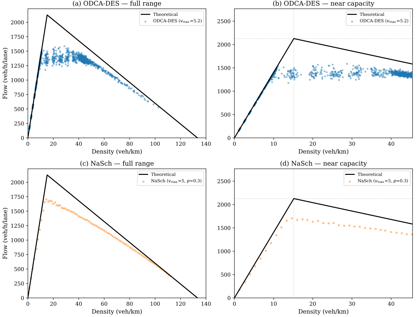
Figure 5: Fundamental diagram validation against the theoretical triangular FD ( v_f = 5.2 cells/s, \tau = 1.5 s, q_{\max} = 2127 veh/h). Top row: ODCA-DES (continuous speeds, v_{\max} = 5.2 ) produces a smooth envelope across (a) the full density range and (b) near capacity, on the theoretical line in free flow and peaking at 1,587.586 veh/h on this open segment ( 1,948-1,948-2,978.041 veh/h on a ring road, see text). Bottom row: NaSch (integer speeds, v_{\max} = 5 , p = 0.3 ) produces clustered flow-density points with a staircase congested branch across (c) the full range and (d) near capacity.
