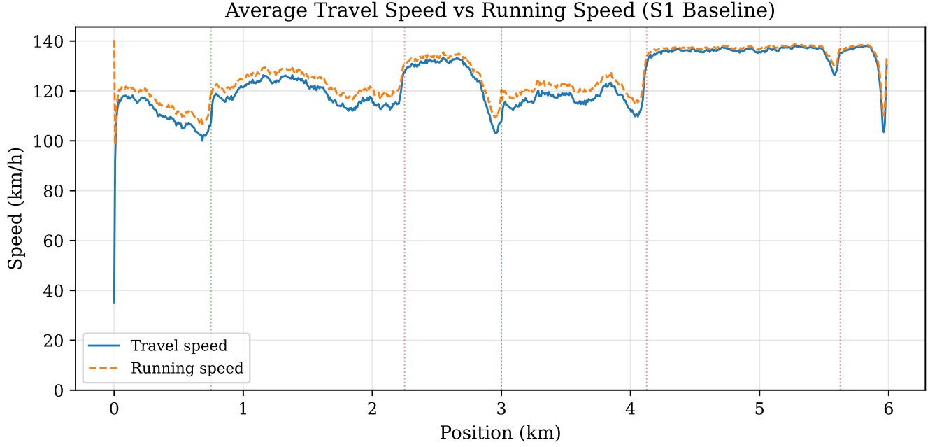
Figure 7: Average travel speed (solid) and running speed (dashed) as a function of position along the freeway (S1, one run). The gap between the two curves is the average cell-level waiting time. Speeds are lowest over the first four kilometres, where ramp traffic and mandatory lane changes concentrate, and recover downstream of off-ramp 2. Dotted lines mark the on-ramps, dashed lines the off-ramps.
