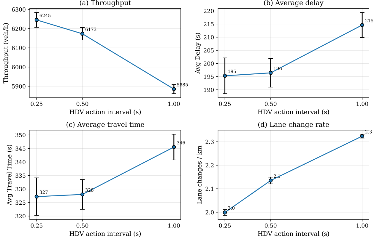
Figure 11: Sensitivity of S1 performance metrics to HDV action interval \delta_{eval} . Panels show throughput, average travel time, average delay, and lane-change frequency. Error bars denote 95% confidence intervals. Reducing the action interval monotonically improves all metrics.
