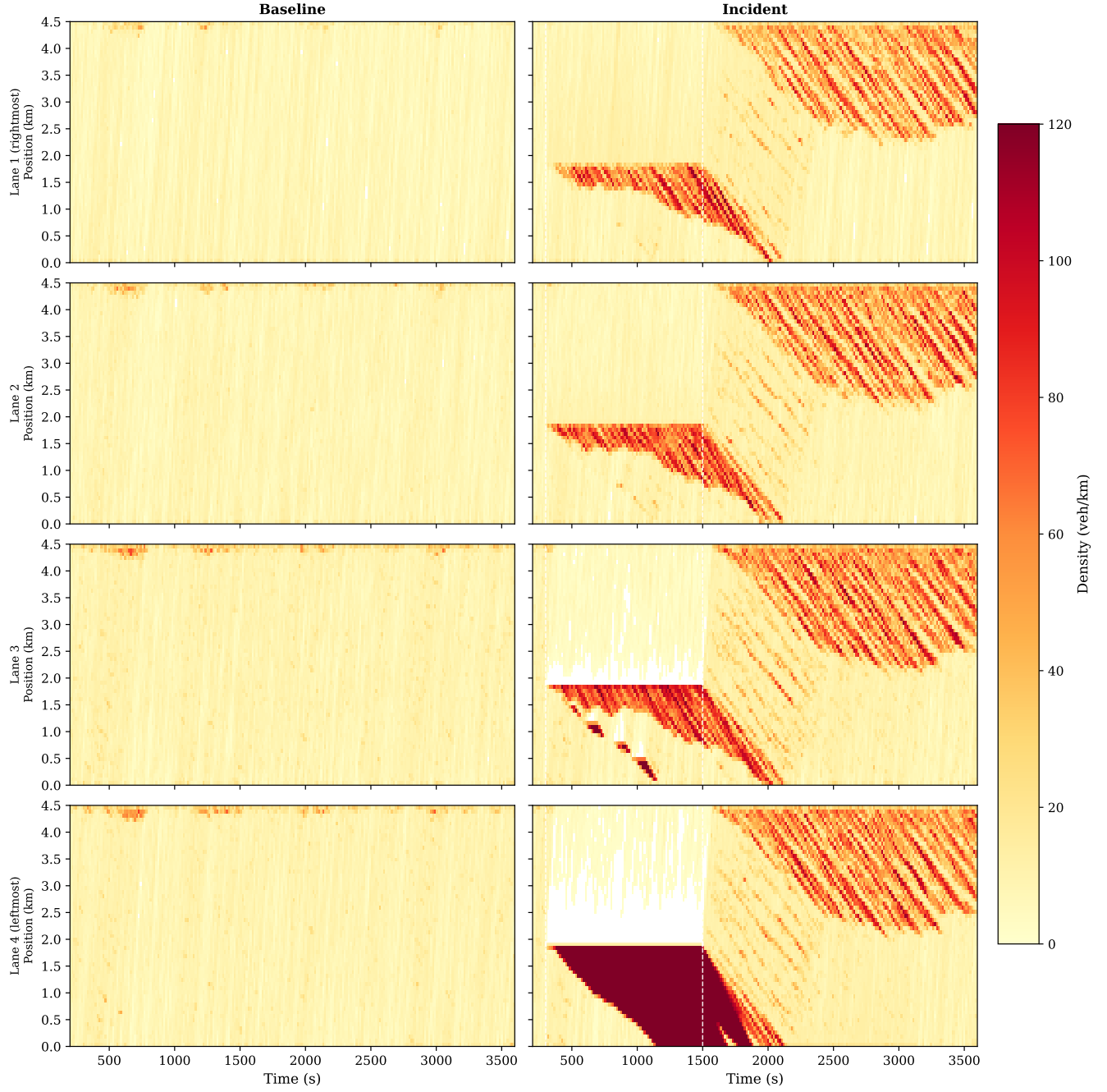
Figure 14: Lane-by-lane time-space density heatmaps ( 15\text{ s} \times 75\text{ m} bins): baseline (left) vs. the 20-minute closure of lanes 3 and 4 (right). White dashed lines on the incident panels mark incident onset ( t = 300\text{ s} ) and clearance ( t = 1500\text{ s} ). The uniform baseline contrasts with lane-specific congestion patterns: lane 4 shows direct blockage impact, while lanes 1–3 show progressive density increases from merging traffic.
