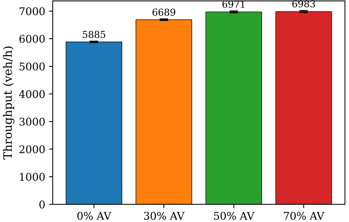
Figure 8: Network throughput and delay across AV penetration scenarios (S1–S4, N = 20 replications). Error bars denote 95% confidence intervals. Throughput increases from 5,891 5,885 to 6,984 6,983 veh/h, saturating at the 7,000 veh/h offered demand, while delay decreases from 215 to 9 s.
