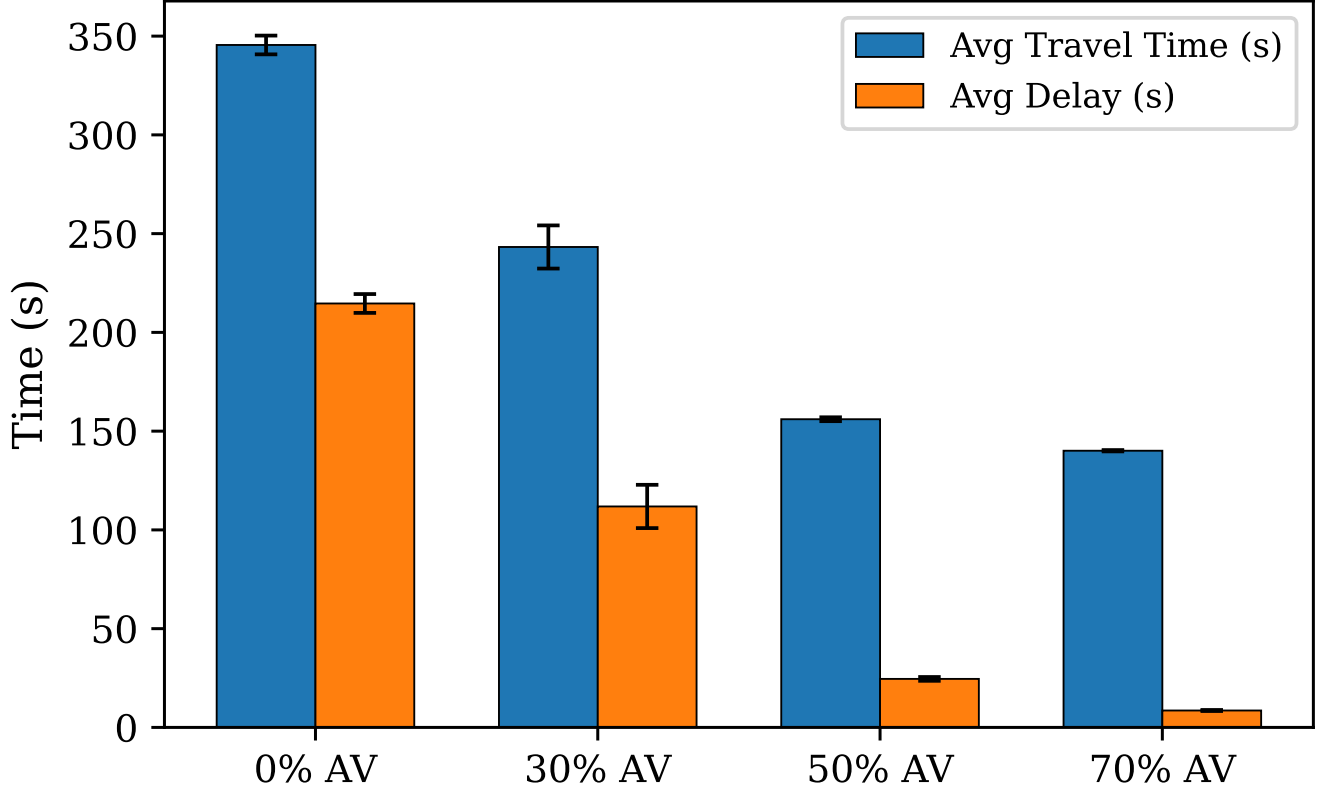
Figure 9: Average travel time across AV penetration scenarios (S1–S4, N = 20 replications). Error bars denote 95% confidence intervals. Travel time decreases from 345 346 s (S1) to 140 s (S4). Trips end at three off-ramps and at the segment end, so the reference is not the full-segment free-flow time of 154 s but the demand-weighted free-flow trip time of 131 s, which S4 exceeds by 7%. The latter is the mean of each origin–destination pair’s free-flow time \ell \Delta c / v_f weighted by its flow (Section 5.1.3); it is shorter than 154 s because most traffic leaves at off-ramps 1 to 3 rather than driving the full 800 cells, and it is reproduced by code/manuscript_numbers.py .
