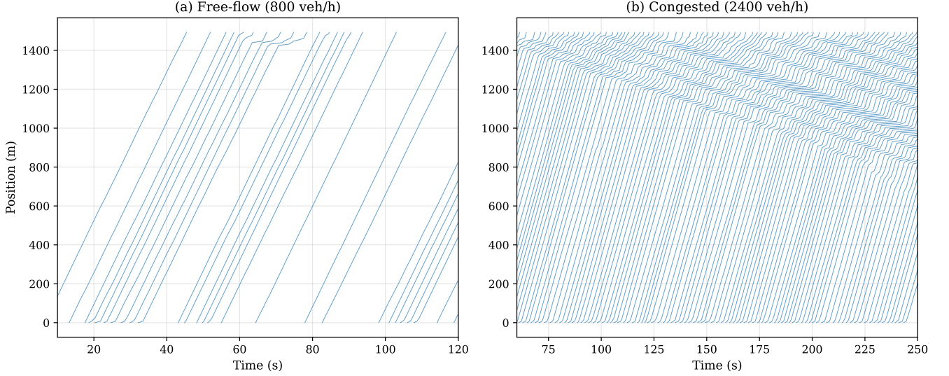
Figure 6: Time-space diagrams on a single-lane segment. (a) Free-flow (800 veh/h): trajectories are near-parallel with slope v_f = 5.2 cells/s ( \approx 140 km/h), with minor perturbations from HDV random slowdowns. (b) Congested (2400 veh/h): trajectory slopes decrease as density exceeds capacity, with backward-propagating waves visible as slope transitions. Trajectories are coloured by each vehicle's average speed (blue above 100 km/h, orange 40–100, red below 40); at this demand every vehicle averages above 100 km/h, and the congestion shows as the bending of individual trajectories rather than as slow vehicles. The disturbances visible in panel (b) travel upstream, the direction the theory gives for w = \ell/\tau = 0.667 cells/s ( \approx 18 km/h).
