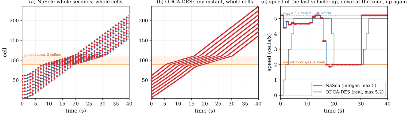
Figure 3: What the two paradigms represent, on the same eight vehicles through the same posted speed-limit zone (shaded, 21 cells at 2 cells/s), both models deterministic (no random slowdown, no driver heterogeneity). The platoon accelerates, slows at the zone and accelerates again, and each follower repeats the move behind the one ahead. (a) NaSch: a red mark is a position, and there is one per vehicle per whole second, each a whole number of cells ahead of the last. (b) ODCA-DES: a red mark is a cell entry, and it occurs at whatever instant the crossing takes; 14 of the 1,328 entries shown fall on a whole second. The cell axis is the same in both. (c) The speed of the last vehicle: NaSch steps through the integers 0 to 5 cells/s, while ODCA-DES passes through 19 distinct values between 1.86 and 5.20, holds the posted 2.00 exactly, and returns to the 5.2 cells/s that the integer model has no way to name. Produced by code/plot_paradigm_comparison.py .
