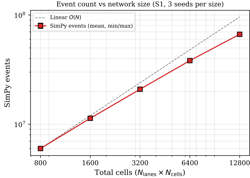
Figure 12: SimPy event count against network size (S1, all-HDV, 3 seeds per size, log-log scale, min to max over seeds as error bars, the dashed line linear growth from the smallest network). The count grows sub-linearly with network length at constant demand (empirical exponent 0.87).
