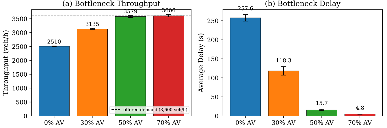
Figure 10: Bottleneck throughput across AV penetration levels ( N = 20 replications). Error bars denote 95% confidence intervals. Throughput rises from 2,503 2,510 to 3,605 3,606 veh/h and flattens between 50% and 70% AV, where the two remaining lanes already carry 99% of the 3,600 veh/h demand (dashed line) and, at 70%, all of it; beyond that point the extra capacity shows up as delay reduction, not as flow.
