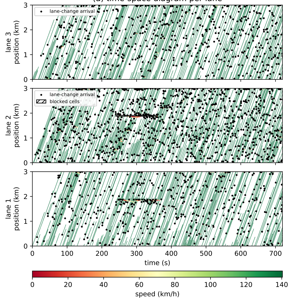
(a) time-space diagram per lane
