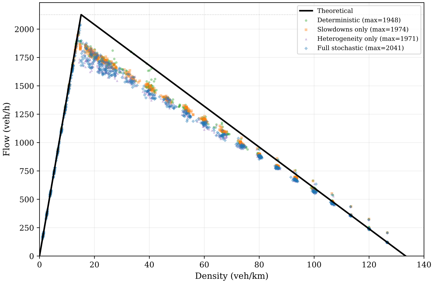
FD Capacity Diagnosis — Ring Road (periodic boundary)
