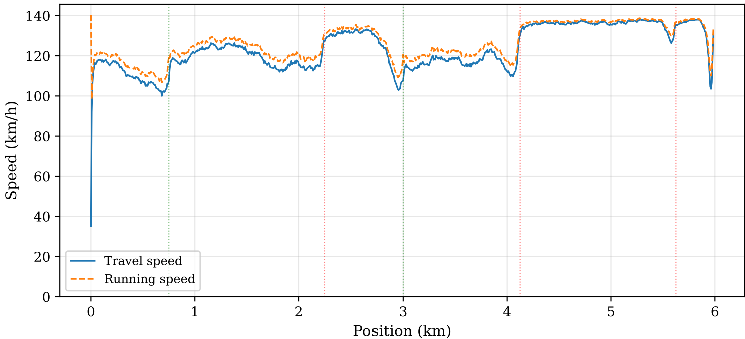
Average Travel Speed vs Running Speed (S1 Baseline)
