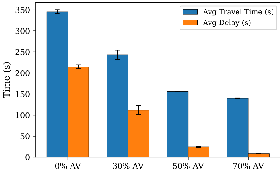
Travel Time and Delay by AV Penetration Rate (mean \pm 95% CI, N=20)
