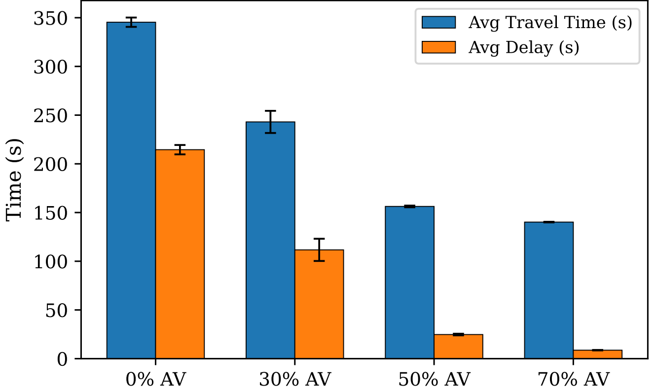
Figure 9: Average travel time across AV penetration scenarios (S1–S4, N = 20 replications). Error bars denote 95% confidence intervals. Travel time decreases from 345 s (S1) to 140 s (S4). Trips end at three off-ramps and at the segment end, so the reference is not the full-segment free-flow time of 154 s but the demand-weighted free-flow trip time of 131 s, which S4 exceeds by 7%. The latter is the mean of each origin–destination pair’s free-flow time \ell \Delta c / v_f weighted by its flow (Section 5.1.3); it is shorter than 154 s because most traffic leaves at off-ramps 1 to 3 rather than driving the full 800 cells, and it is reproduced by code/manuscript_numbers.py .
