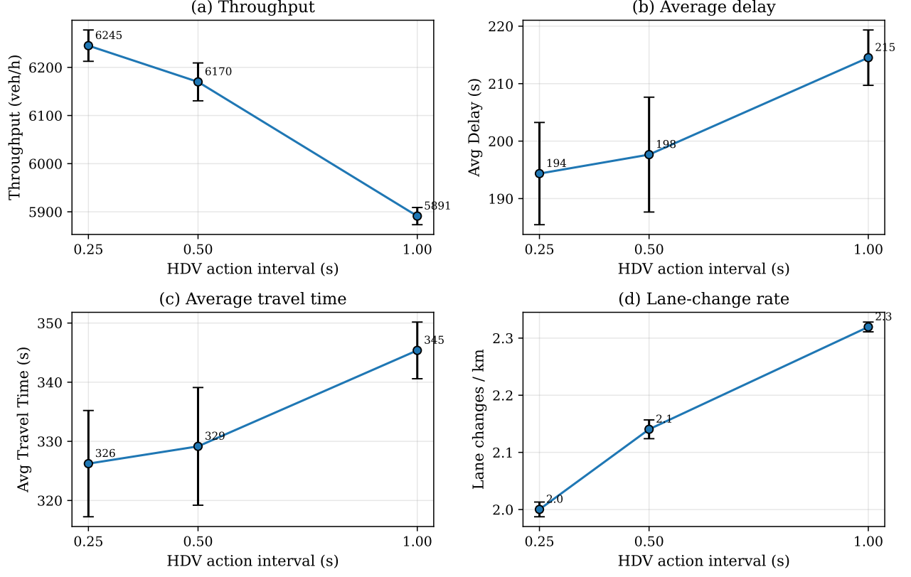
Figure 11: Sensitivity of S1 performance metrics to HDV action interval \delta_{\text{eval}} . Panels show throughput, average travel time, average delay, and lane-change frequency. Error bars denote 95% confidence intervals. Reducing the action interval monotonically improves all metrics.
