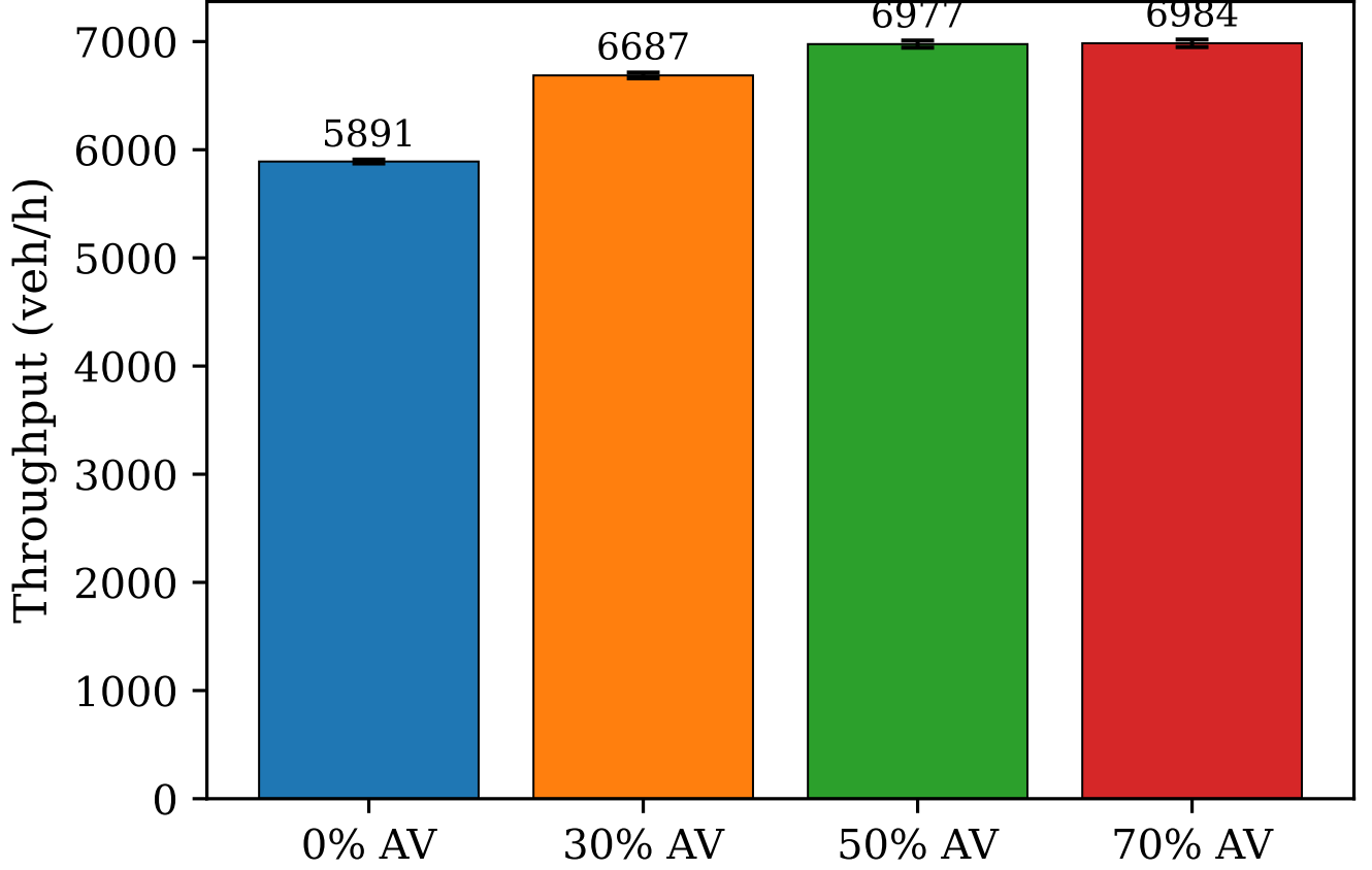
Figure 8: Network throughput and delay across AV penetration scenarios (S1-S4, N = 20 replications). Error bars denote 95% confidence intervals. Throughput increases from 5,891 to 6,984 veh/h, saturating at the 7,000 veh/h offered demand, while delay decreases from 215 to 9 s.
