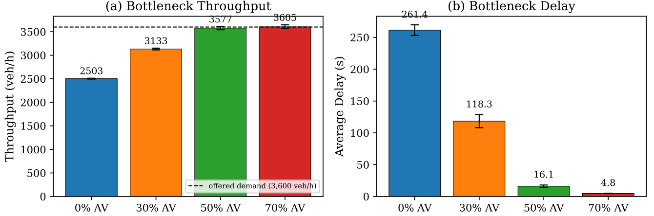
Figure 10: Bottleneck throughput across AV penetration levels ( N = 20 replications). Error bars denote 95% confidence intervals. Throughput rises from 2,503 to 3,605 veh/h and flattens between 50% and 70% AV, where the two remaining lanes already carry 99% of the 3,600 veh/h demand (dashed line) and, at 70%, all of it; beyond that point the extra capacity shows up as delay reduction, not as flow.
