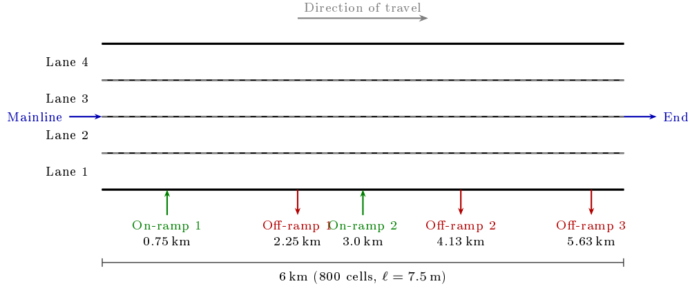
Figure 4: Test network geometry: 4-lane unidirectional freeway segment (6 km, 800 cells at \ell = 7.5 m). On-ramps merge into lane 1 (rightmost); off-ramps exit from lane 1. Mainline demand enters at the first cell of each lane; traffic bound for the segment end is spread over the four lane ends (cell 800), so it crosses lanes in both directions.
