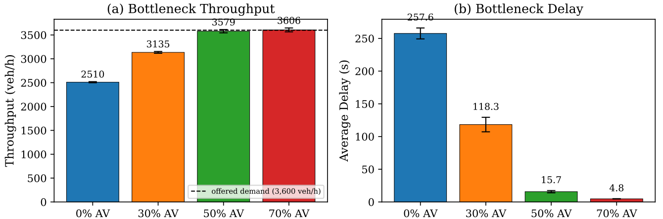
Figure 10: Bottleneck throughput across AV penetration levels ( N = 20 replications). Error bars denote 95% confidence intervals. Throughput rises from 2,510 to 3,606 veh/h and flattens between 50% and 70% AV, where the two remaining lanes already carry 99% of the 3,600 veh/h demand (dashed line) and, at 70%, all of it; beyond that point the extra capacity shows up as delay reduction, not as flow.
