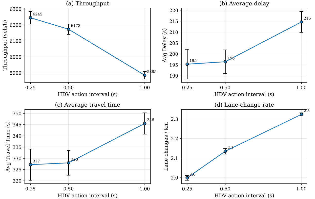
Sensitivity to HDV action interval (Scenario S1, 0% AV; mean \pm 95% CI; N=10 at ai=0.25, N=10 at ai=0.5, N=20 at ai=1.0)
