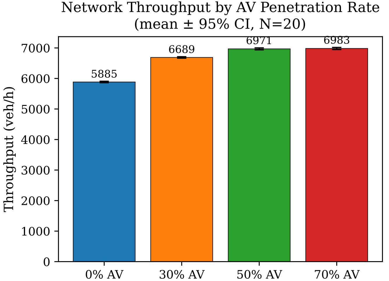
Figure 8: Network throughput across AV penetration scenarios (S1–S4, N = 20 replications). Error bars denote 95% confidence intervals. Throughput increases from 5,885 to 6,983 veh/h, saturating at the 7,000 veh/h offered demand.
