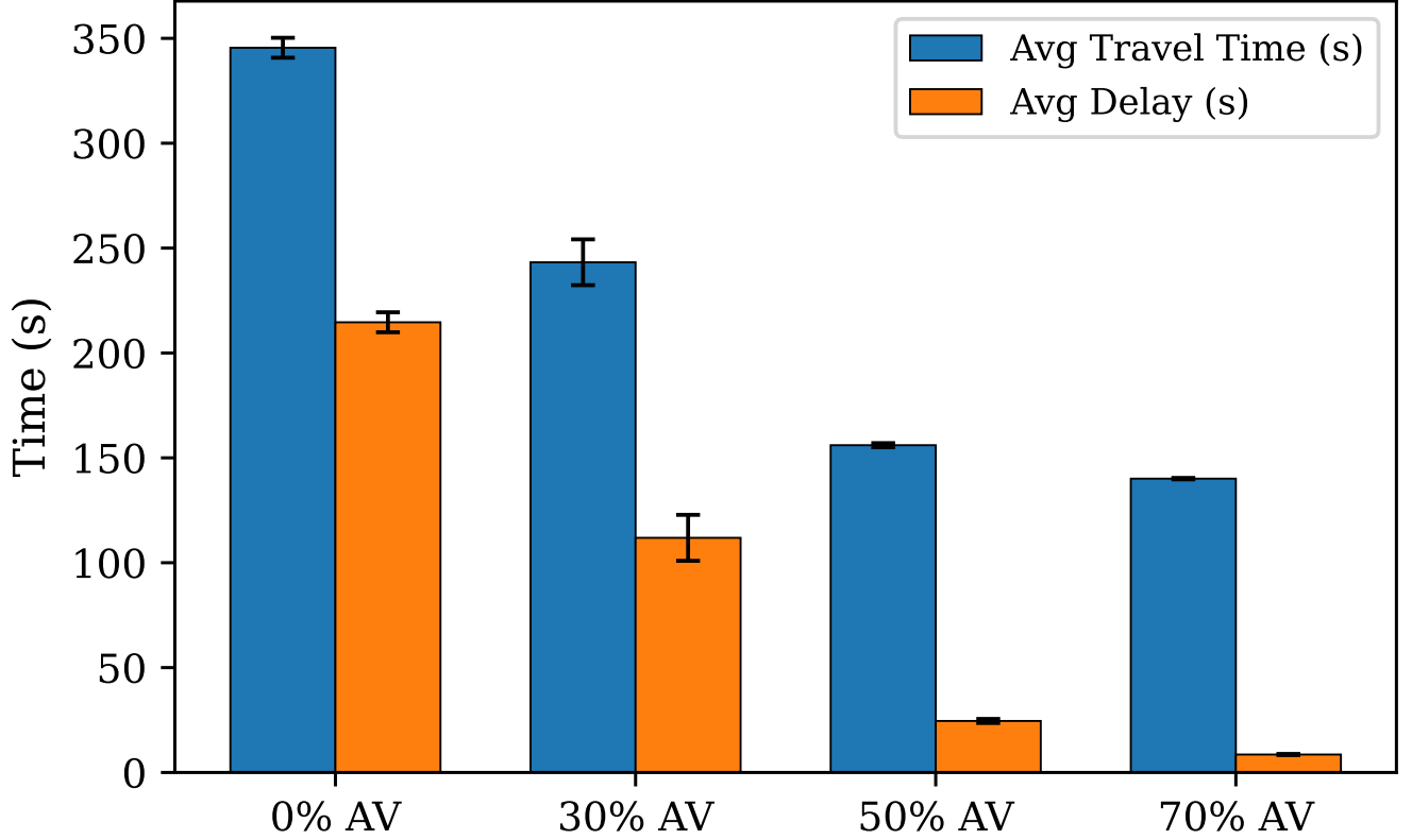
Figure 9: Average travel time across AV penetration scenarios (S1–S4, N = 20 replications). Error bars denote 95% confidence intervals. Travel time decreases from 346 s (S1) to 140 s (S4). Trips end at three off-ramps and at the segment end, so the reference is not the full-segment free-flow time of 154 s but the demand-weighted free-flow trip time of 131 s, which S4 exceeds by 7%. The latter is the mean of each origin–destination pair’s free-flow time \ell \Delta c / v_f weighted by its flow (Section 5.1.3); it is shorter than 154 s because most traffic leaves at off-ramps 1 to 3 rather than driving the full 800 cells, and it is reproduced by code/manuscript_numbers.py .
