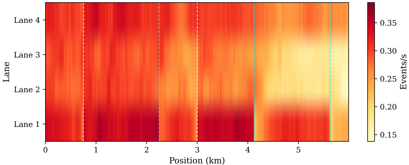
Event Density (events/s/cell)
