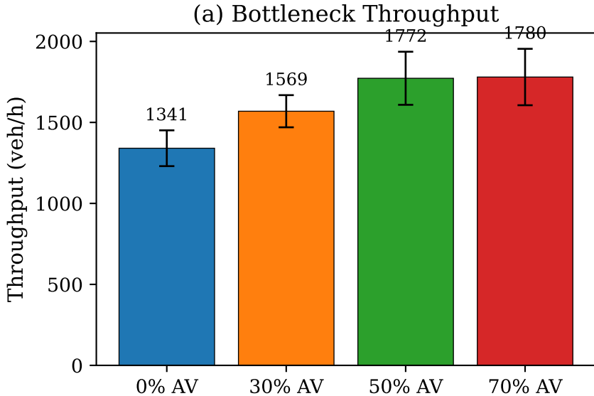
Bottleneck: Throughput and Delay by AV Penetration (mean \pm 95% CI, N=20)
