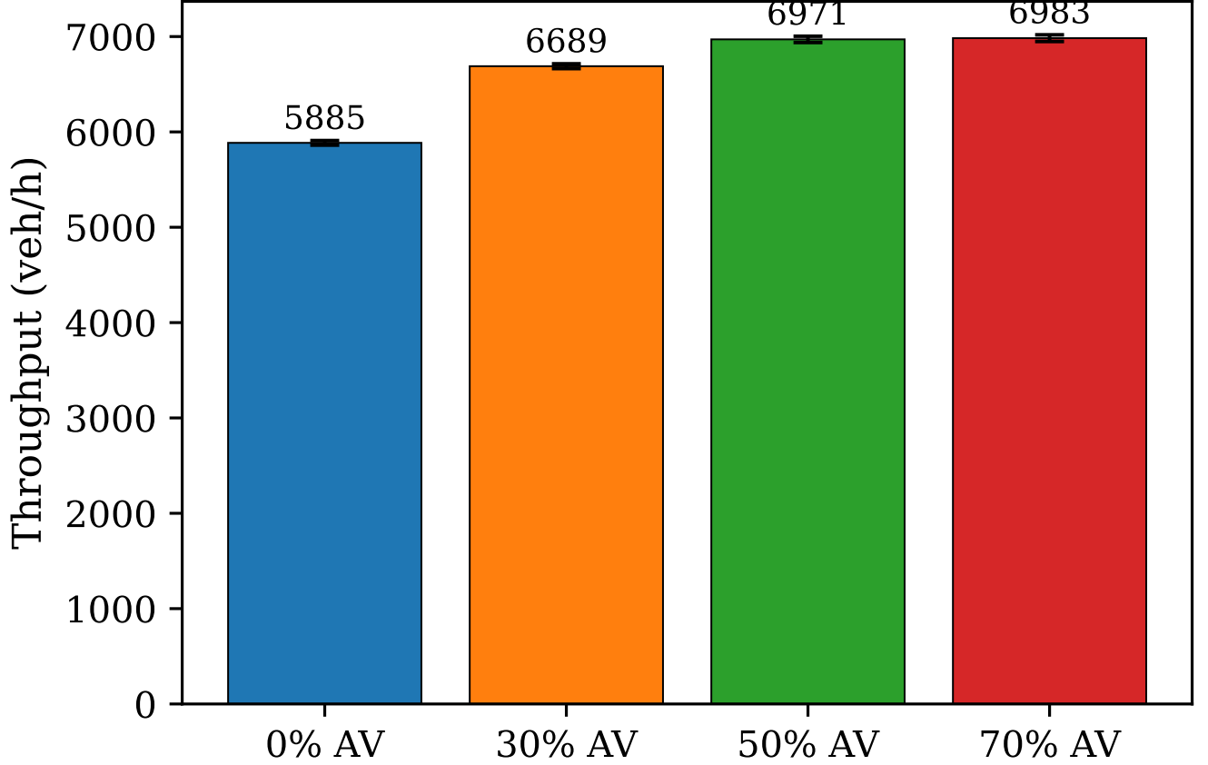
Figure 8: Network throughput across AV penetration scenarios (S1–S4, N = 20 replications). Error bars denote 95% confidence intervals. Throughput increases from 5,885 to 6,983 veh/h, saturating at the 7,000 veh/h offered demand.
